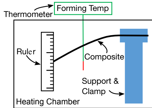
Figure M293-4. Bending test setup [3]
