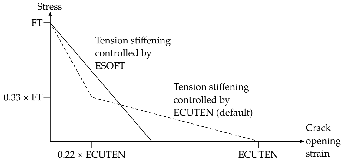
Figure M172-1. Tensile Behaviour of Concrete
