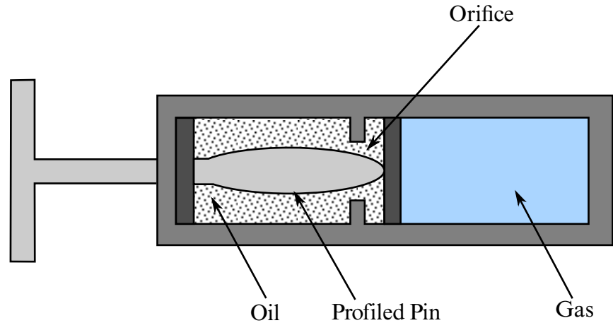
Figure M70-1. Schematic of Hydraulic/Gas damper.
