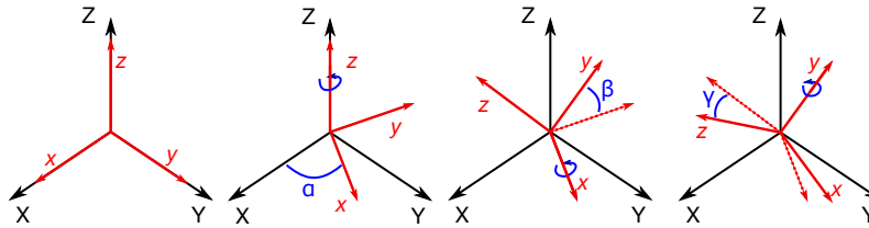
Figure 7-4. A rotation represented by Tait-Bryan angles (\alpha, \beta, \gamma) using Z(\alpha)X(\beta)Y(\gamma) intrinsic rotations
