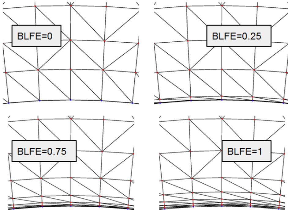
Figure 8-2. BLST = 2 example
