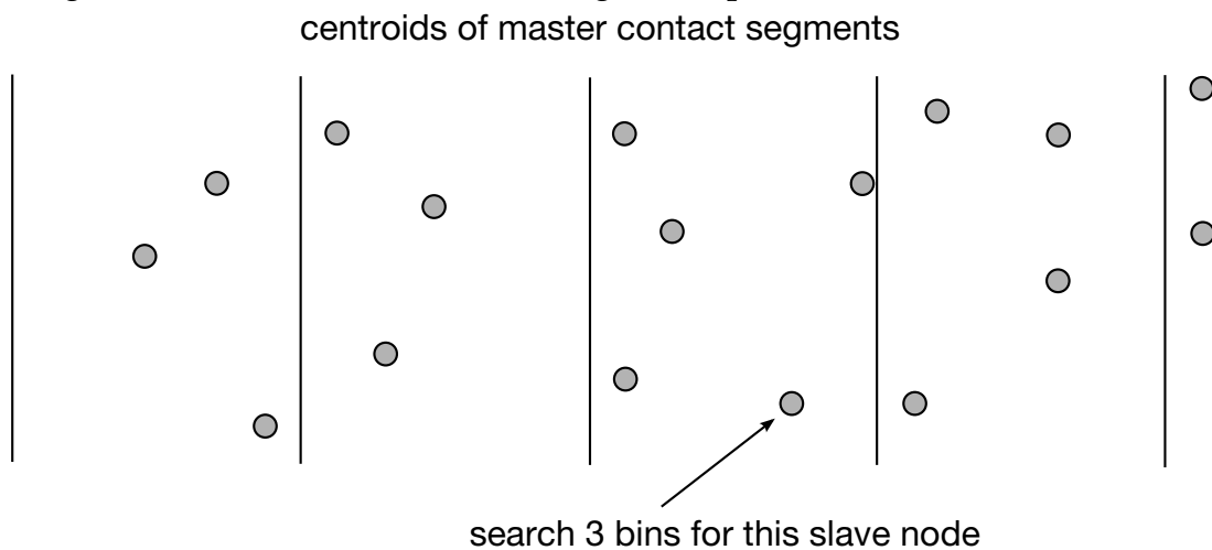
Figure 29.8. One-dimensional bucket sorting identifies the nearest segments for each slave node.
