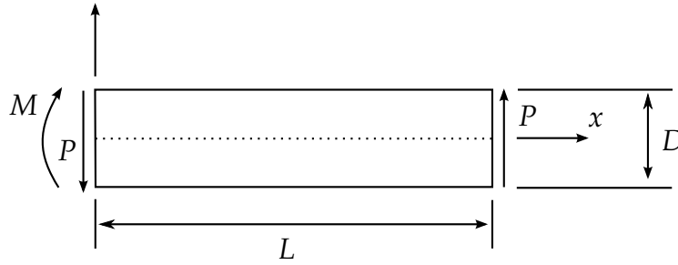
Figure 16.4. Timoshenko cantilever beam.
