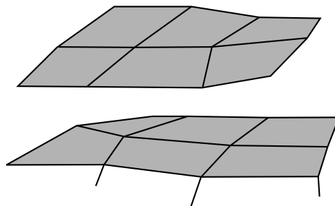
Figure 29.12. The slave and master surfaces must be offset in the input by one-half the total shell thickness. This also allows the segments to be oriented automatically.
