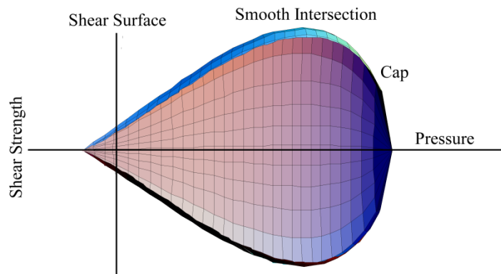
Figure 22.159.1. General Shape of the concrete model yield surface in two-dimensions.
