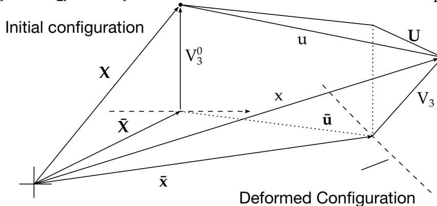
Figure 43.5. Deformation of a shell.
