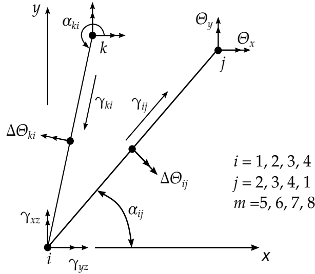
Figure 44.3. Nodal and edge shear strains [Wilson 2000].
