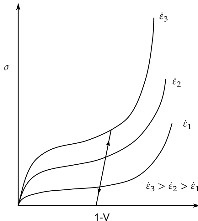
Figure 22.83.1. Rate effects in Fu Chang's foam model.
