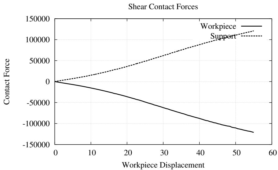
Figure 29-47 A rubber compression example solved in implicit with Mortar contact (Courtesy of Dellner Couplers AB). The graph shows the contact force between the rubber parts and the moving workpiece and between the rubber parts and the two supports, respectively.
