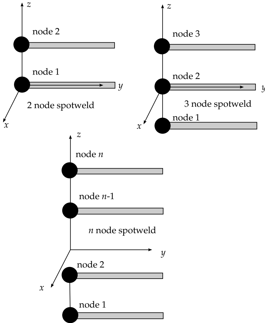
Figure 28.2. Nodal ordering and orientation of the local coordinate system is important for determining spotweld failure.
