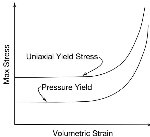
Figure 22.75.1. Behavior of crushable foam. Unloading is elastic.
