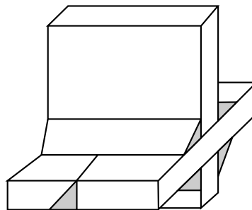
Figure 28.6. A general weld is a mixture of fillet and butt welds.
