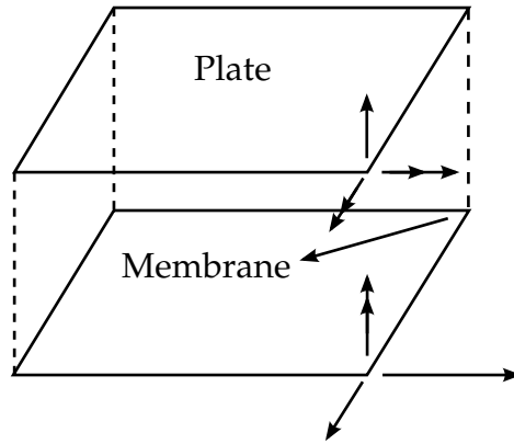
Figure 44.1. Shell as assembly of plate and membrane elements
