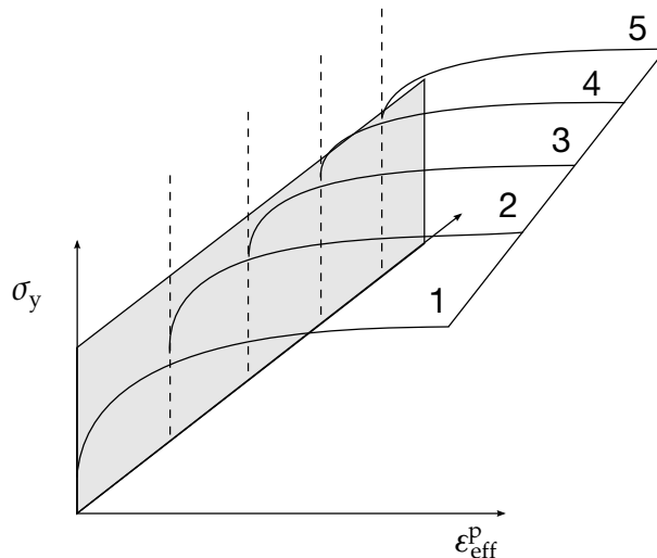
Figure 22.25.1. Rate effects may be accounted for by defining a table of curves.
