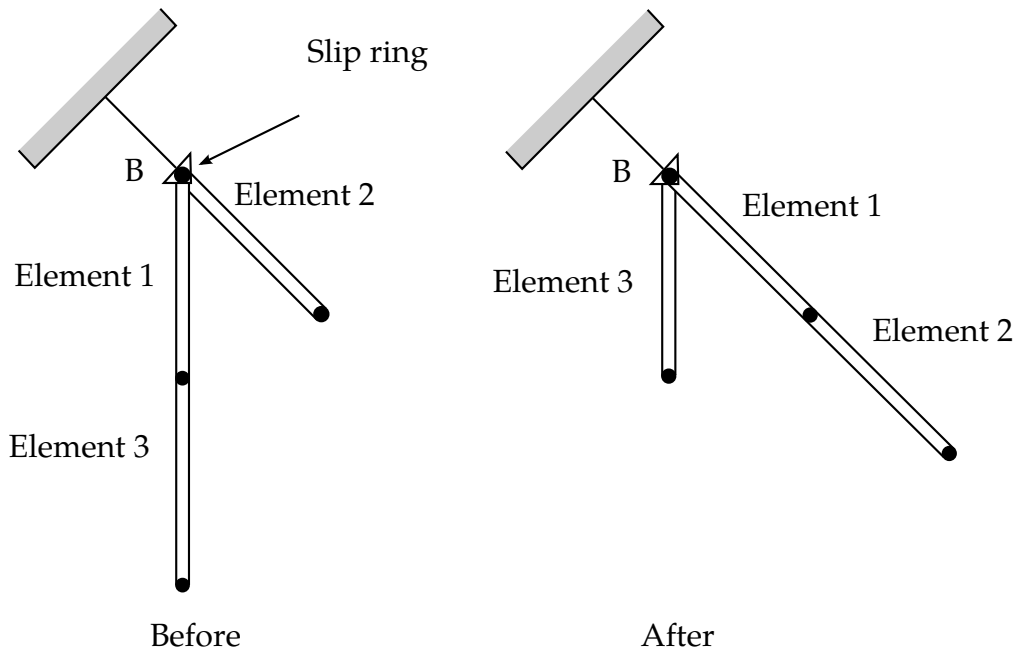
Figure 19.7. Elements passing through slipping.
