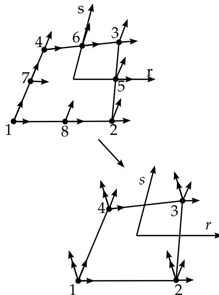
Figure 44.4. Eight node membrane element.
