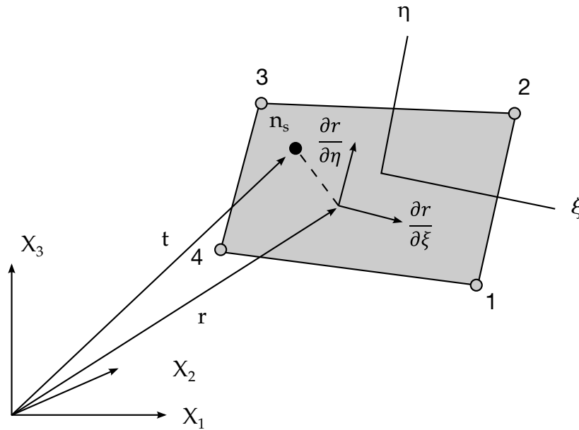
Figure 29.6. Location of contact point when n_s lies above master segment.
