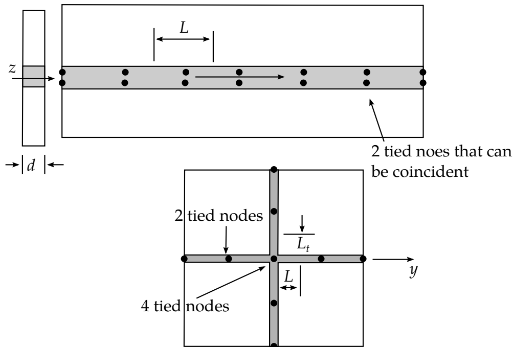
Figure 28.4. Orientation of the local coordinate system and nodal ordering is shown for butt weld failure.
