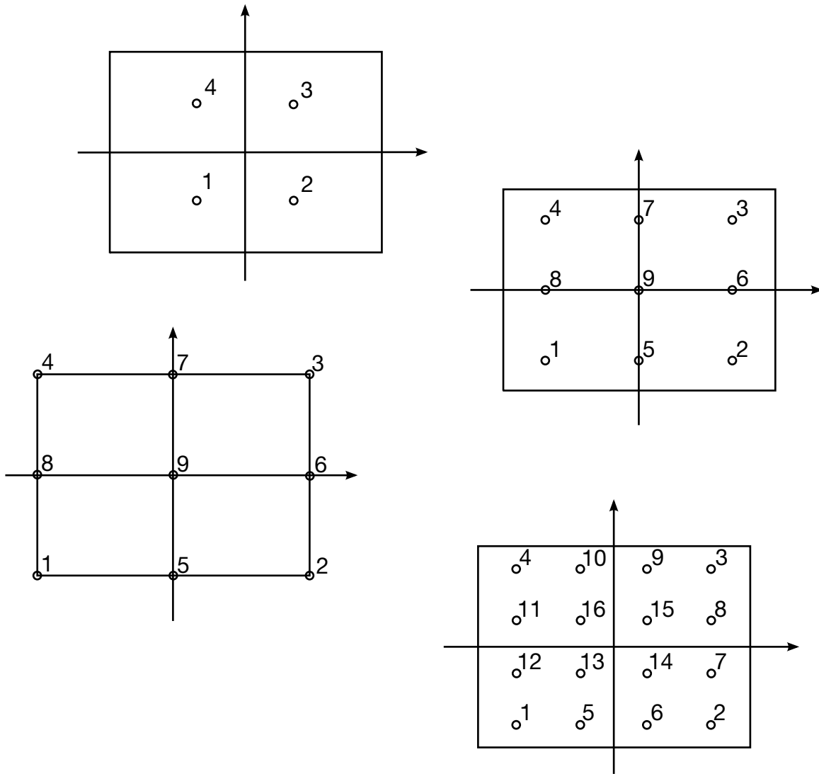
Figure 7.3. Integration possibilities for rectangular cross sections in the Hughes-Liu beam element.
