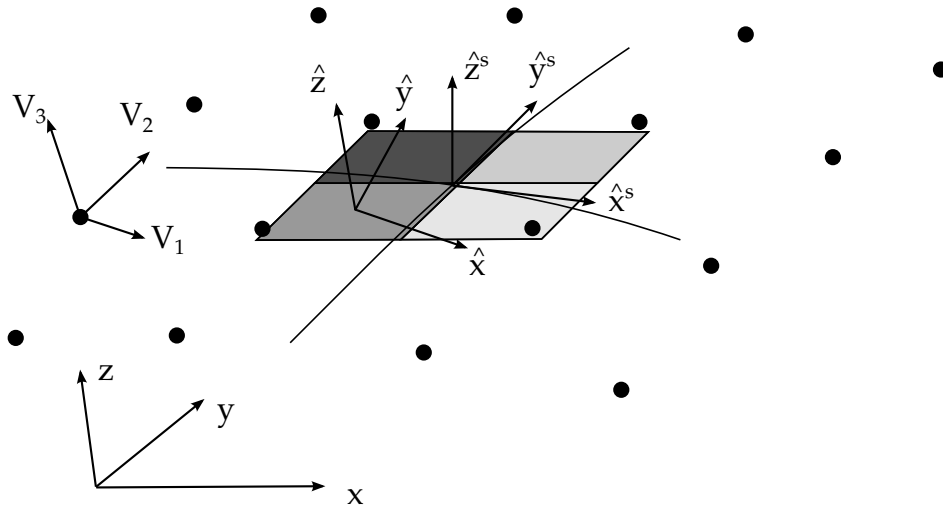
Figure 43.6. Local co-rotational and nodal coordinate systems.
