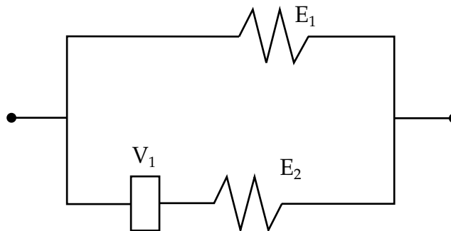
Figure 22.62.1. Schematic of Material Model 62.
