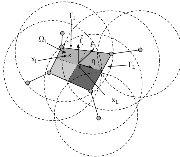
Figure 43.7. Integration scheme for mesh-free shells.
