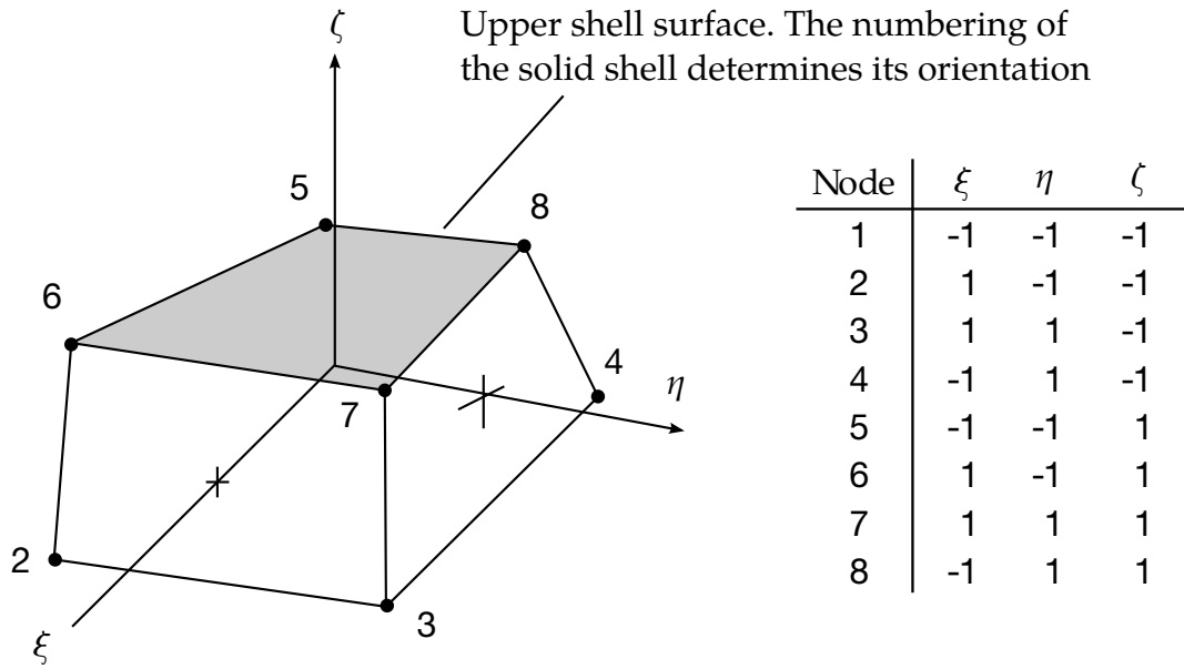
Figure 15.1. Eight node solid shell element
