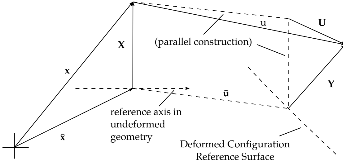
Figure 13.2. Schematic of deformed configuration displacements and position vectors.
