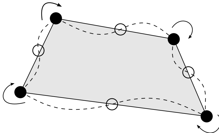
Figure 44.6. Zero energy mode
