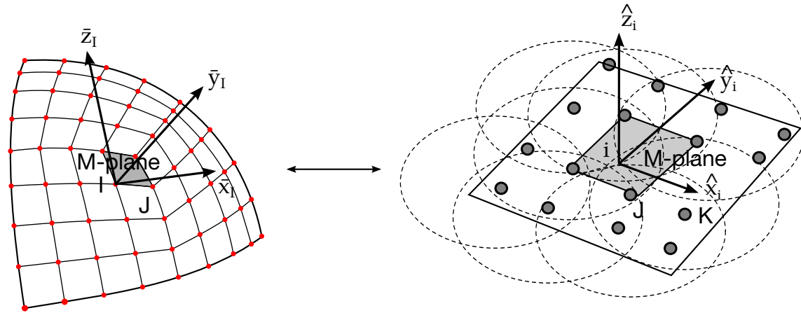
Figure 43.3. Mesh-free shell local projection
