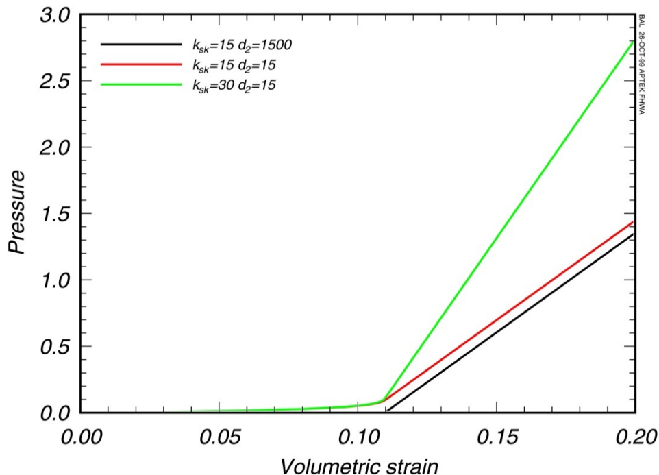
Figure 22.147.3. The effects of D_2 and K_{sk} parameters on pore water pressure.
