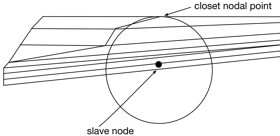
Figure 29.7. Failure to find the contact segment can be caused by poor aspect ratios in the finite element mesh.
