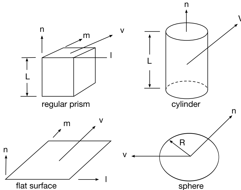
Figure 29.30. Vector n determines the orientation of the generalized stonewalls. For the prescribed motion options the wall can be moved in the direction V as shown.
