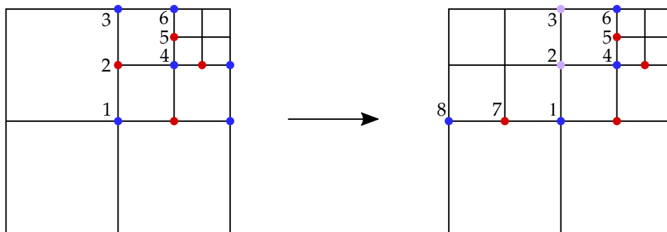
Figure 36.10. Illustration of which nodes are constrained after the element to the left of Node 2 is adapted. The purple nodes indicate which ones are no longer part of constraints.
