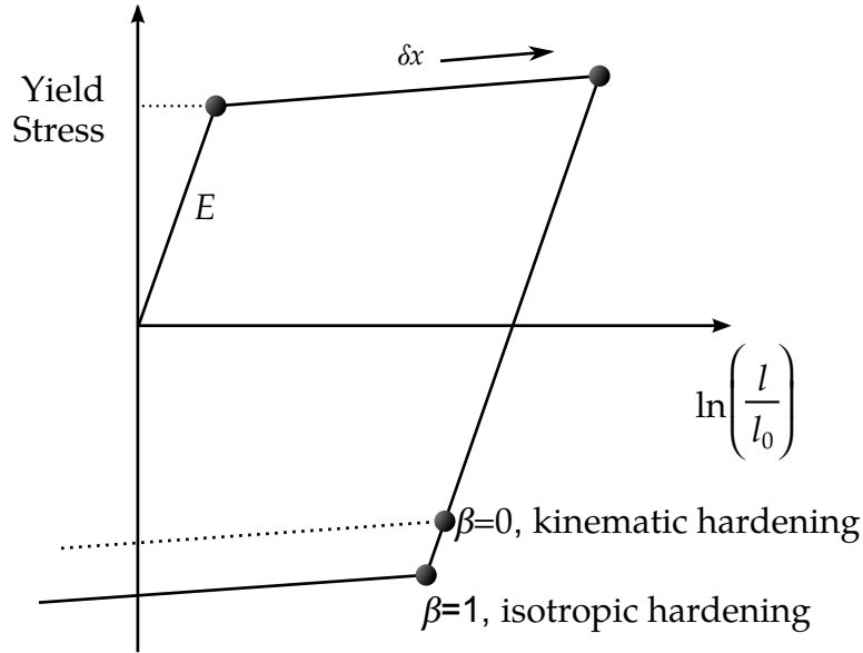
Figure 22.3.1. Elastic-plastic behavior with isotropic and kinematic hardening where l_0 and l are the undeformed and deformed length of uniaxial tension specimen, respectively.
