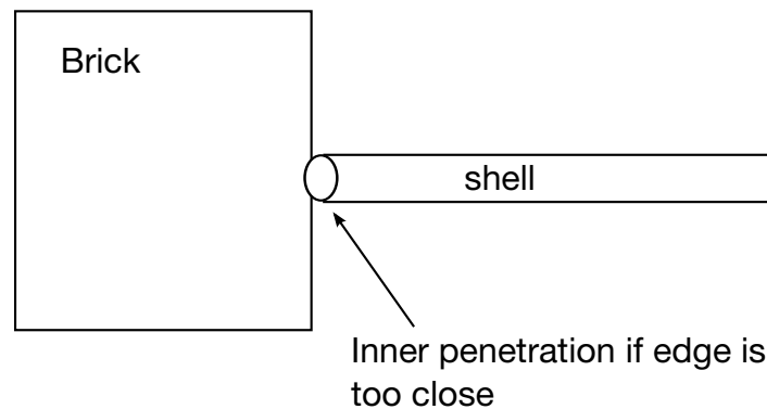
Figure 29.15. Undetected interpenetration due to rounding the edge of the shell element.
