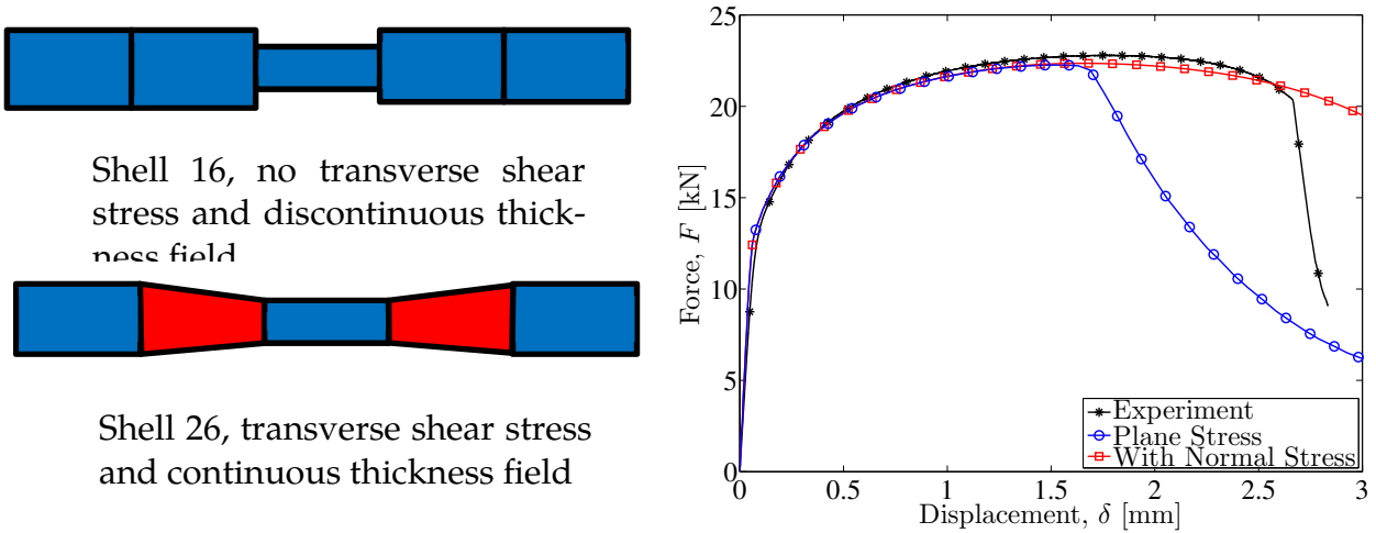
Figure 1212-1 Example of premature localization with shell type 16 while shell type 26 matches experimental result (from Björklund)
