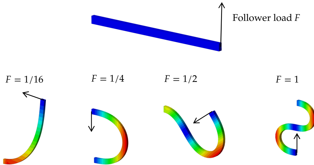
Figure 3737-3 Nonlinear implicit solution of an elastic cantilever beam with a follower force, von Mises stress is fringed..
