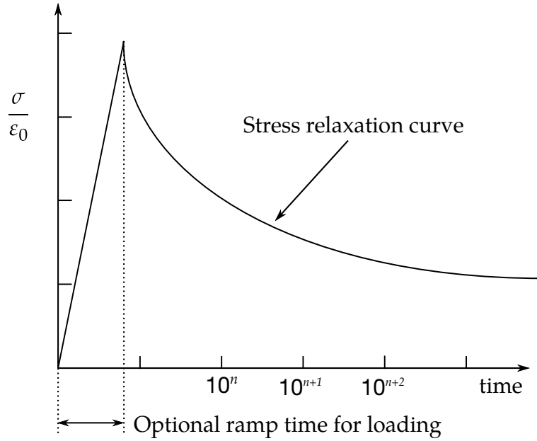
Figure 22.76.1. Relaxation curve. This curve defines stress versus time where time is defined on a logarithmic scale. For best results, the points defined in the load curve should be equally spaced on the logarithmic scale. Furthermore, the load curve should be smooth and defined in the positive quadrant. If nonphysical values are determined by least squares fit, LS-DYNA will terminate with an error message after the initialization phase is completed. If the ramp time for loading is included, then the relaxation which occurs during the loading phase is taken into account. This effect may or may not be important.
