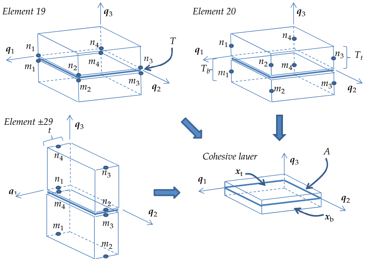
Figure 5.1. Illustration of cohesive elements 19, 20 and \pm 29
