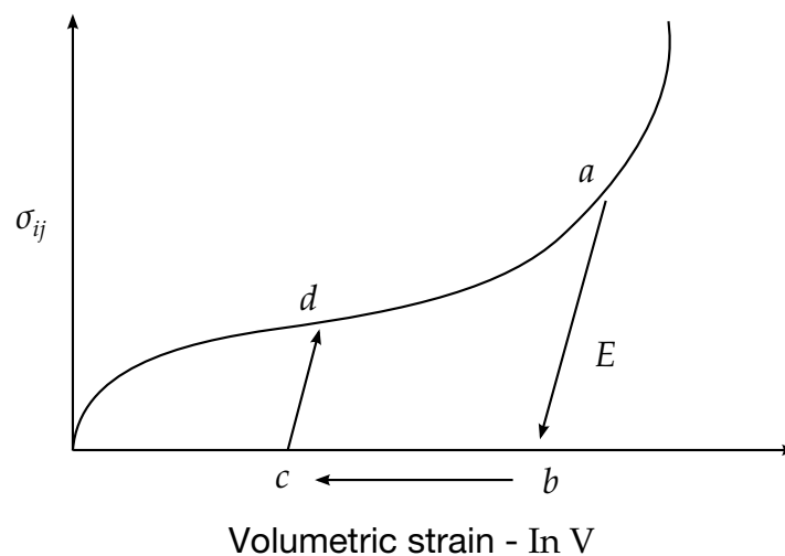
Figure 22.63.1. Yield stress versus volumetric strain curve for the crushable foam.
