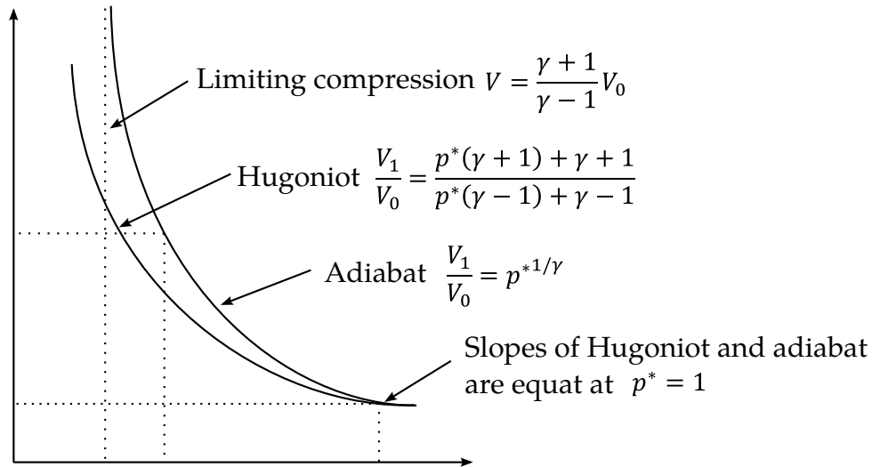
Figure 24.3. Hugoniot curve and adiabat for a g-law gas (from [Noh 1976]).
