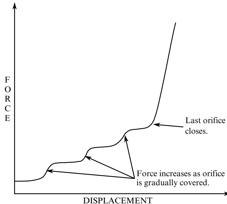
Figure 22.69.2. Force versus displacement as orifices are covered at a constant relative velocity. Only the linear velocity term is active.
