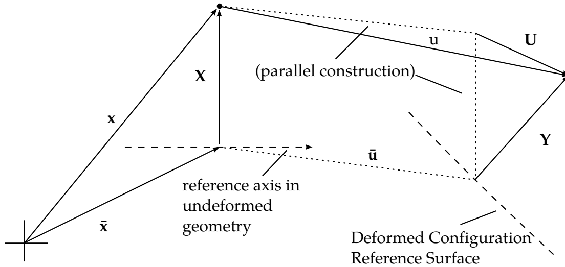
Figure 7.2. Schematic of deformed configuration displacements and position vectors.
