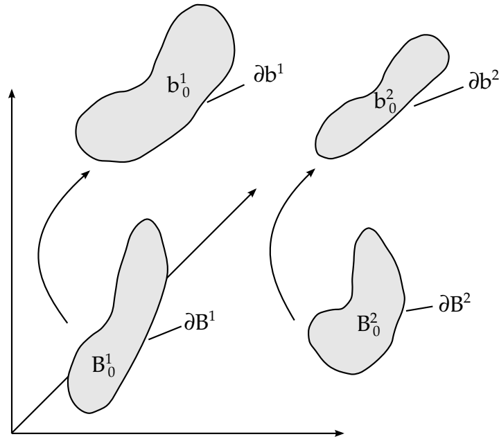
Figure 29.2. Reference and deformed configuration.
