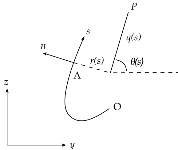
Figure 8.1. Definition of coordinates in thin-walled open section
