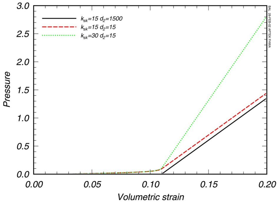
Figure 22.147.1. Pressure versus volumetric strain showing the effects of D1 parameter.
