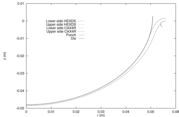
Figure 16.10. Deformed shape of a circular sheet with punch travel 50 mm
