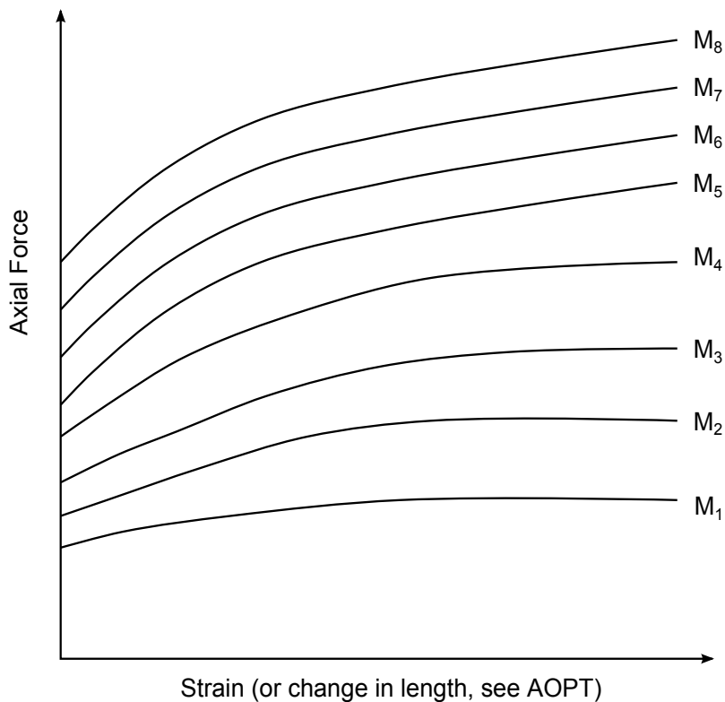
Figure 22.139.1. The force magnitude is limited by the applied end moment. For an intermediate value of the end moment LS-DYNA interpolates between the curves to determine the allowable force value.
