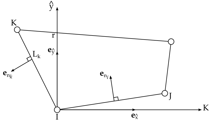
Figure 9.4. Vector and edge definitions for computing the transverse shear strain components.
