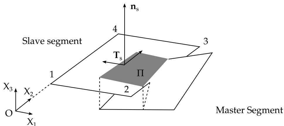
Figure 29.41. Illustration of Mortar segment to segment contact
