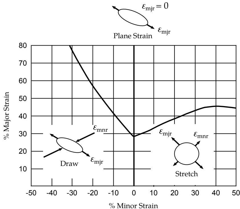
Figure 22.39.1. Flow limit diagram.
