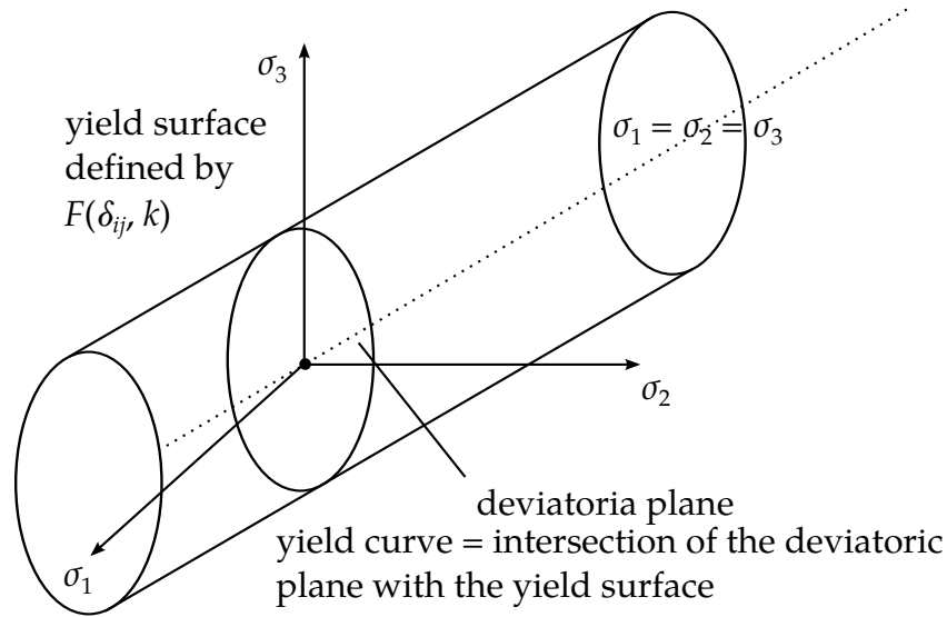
Figure 21.2. The yield surface in principal stress space in pressure independent.
