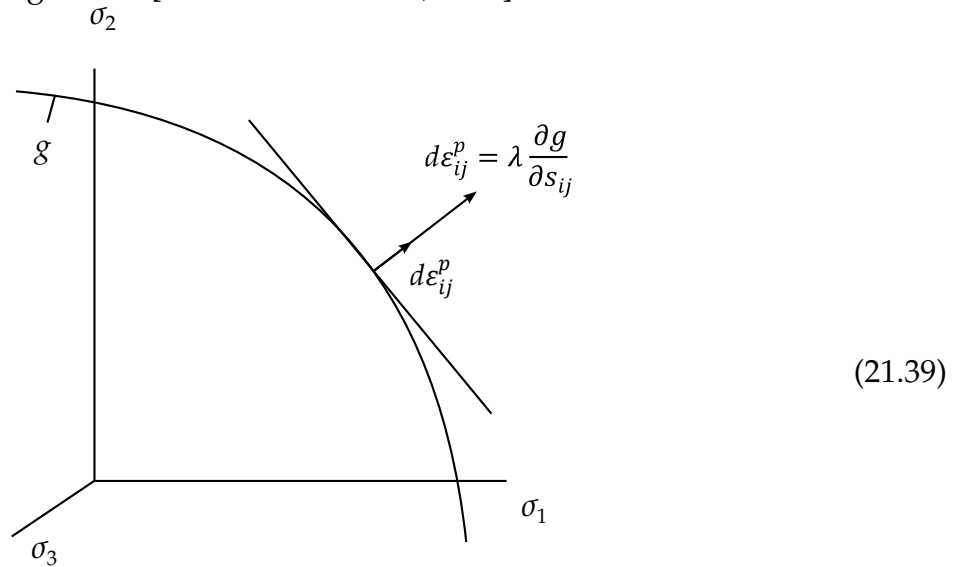
Figure 21.5. The plastic strain is normal to the yield surface.
