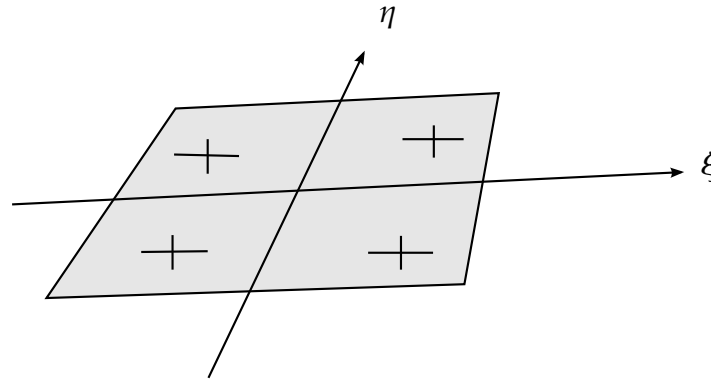
Figure 13.5. Selectively reduced integration rule results in four inplane points being used.
