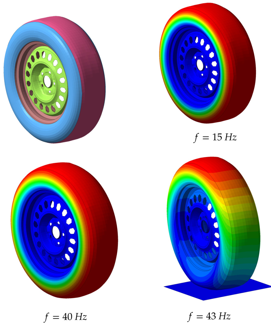
Figure 37.5. Intermittent eigenvalue analysis of tire. Model shown in top left, followed by lowest frequency modes for unpressurized tire (top right), inflated tire (bottom left) and inflated tire and frictional contact (bottom right). Resultant mode displacements are fringed.
