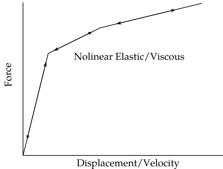
Figure 19.1. Piecewise linear force-displacement curve for nonlinear elastic discrete element.
