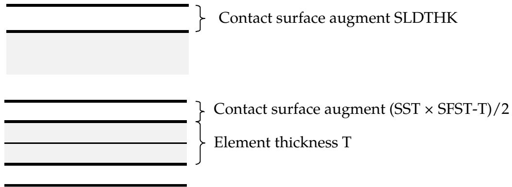
Figure 29.45. Illustration of contact surface location for automatic Mortar contact, solids on top and shells below.
