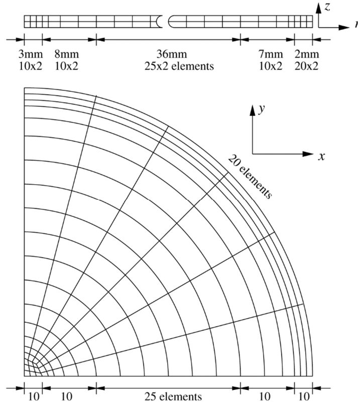
Figure 16.9. Mesh for circular sheet stretching
