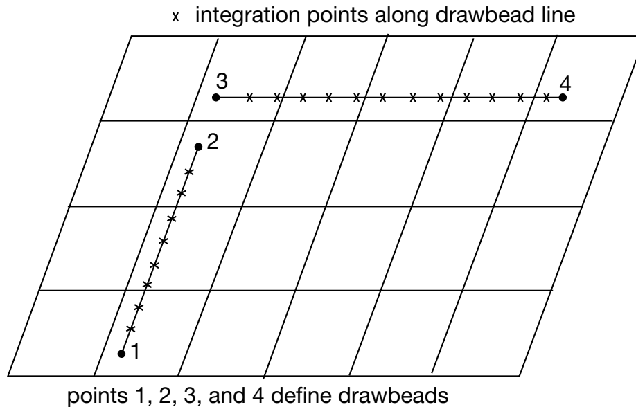
Figure 29.33. The drawbead contact provides a simple way of including drawbead behavior without the necessity of defining a finite element mesh for the drawbeads. Since the draw bead is straight, each bead is defined by only two nodes.
