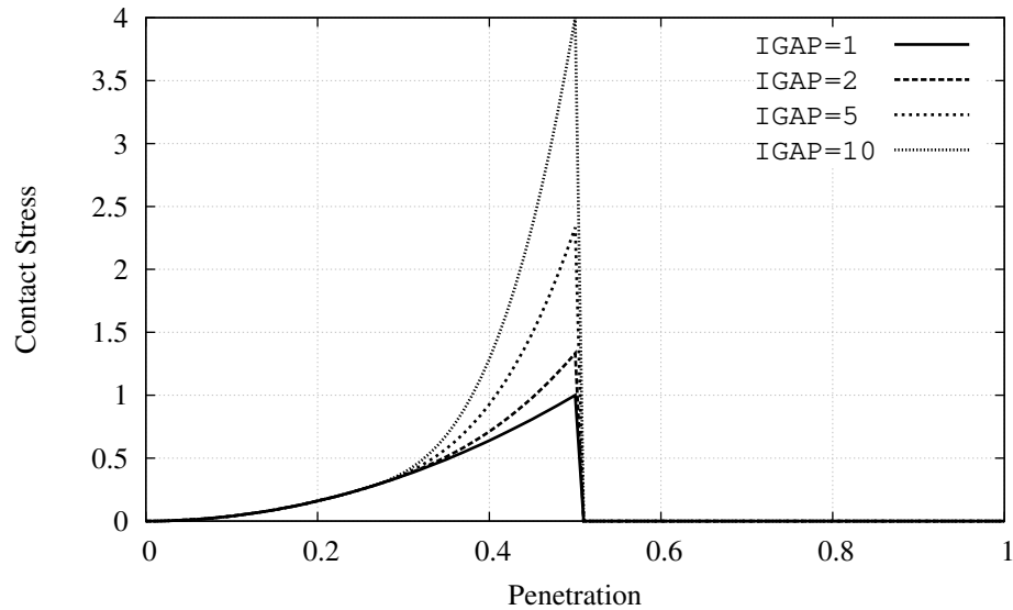
Figure 29.44. Mortar contact stress as function of penetration relative 2d_{\max} .
