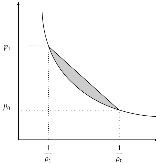
Figure 24.2. Shocking takes place along the Rayleigh line, and release closely follows the Hugoniot. The cross-hatched area is the difference between the internal energy behind the shock and the internal energy lost on release.
