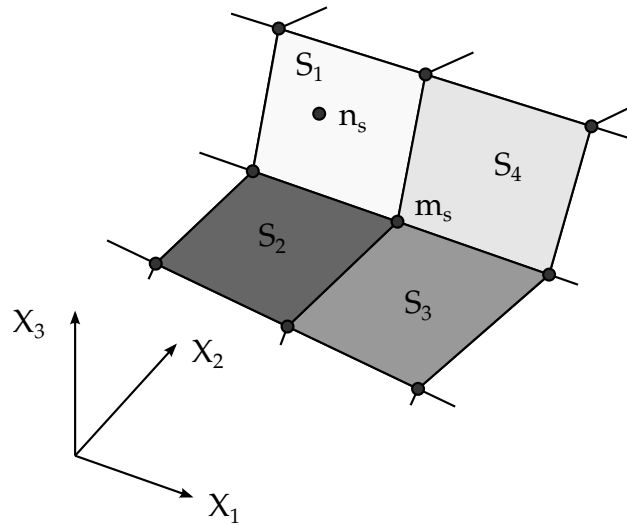
Figure 29.3. In this figure, four master segments can harbor slave node n_s given that m_s is the nearest master node.
