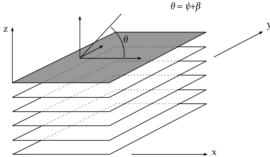
Figure 21.7. A multi-layer laminate can be defined. The angle \beta_i is defined for the i th lamina.
