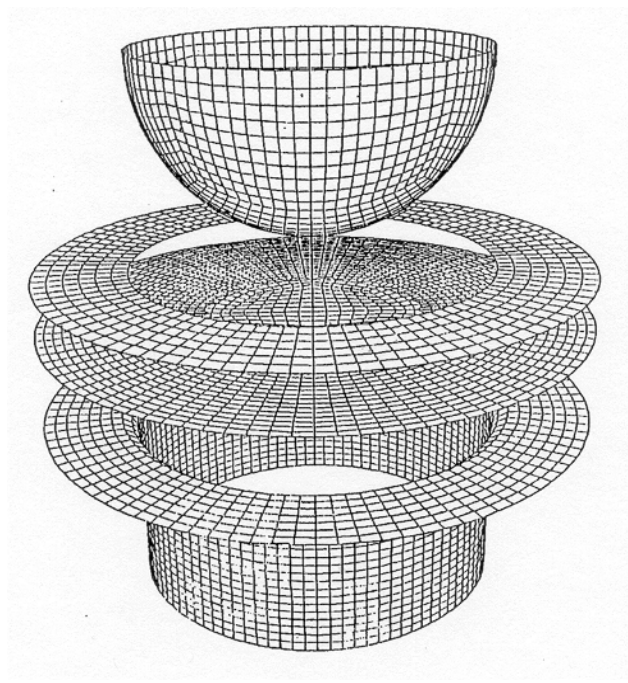
Figure 29.16. Hemispherical deep drawing problem.
