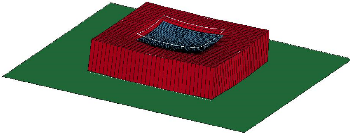
Figure 1212-3 Compression of a shell sheet between two rigid plates using IDOF = 3 on shell 16.
