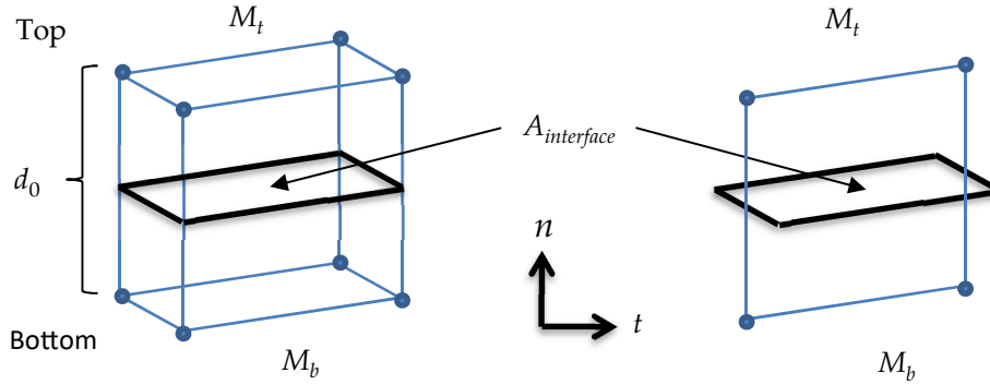
Figure 25.2. Solid and shell cohesive element with initial separation d_0 and total top and bottom nodal masses M_t and M_b . The interface area of the shell element is defined using the shell thickness.
