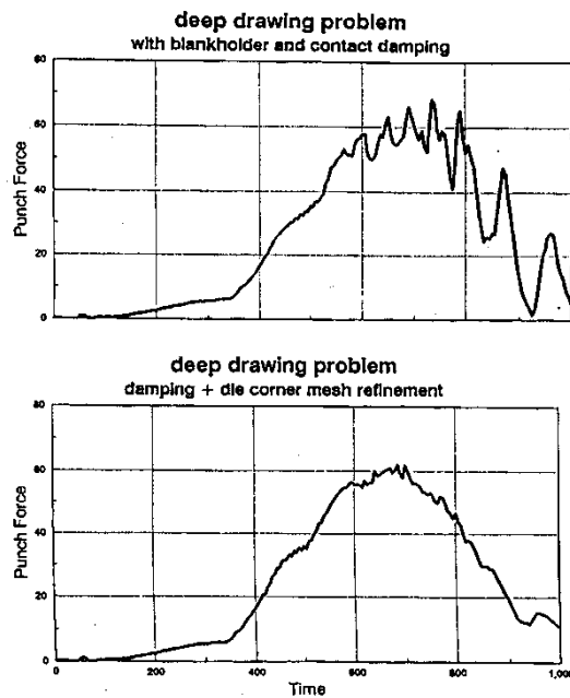
Figure 29.19. The oscillations are effectively eliminated by the mesh refinement.
