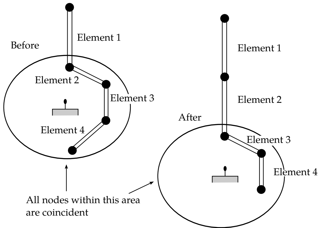
Figure 19.8. Elements in a retractor.
