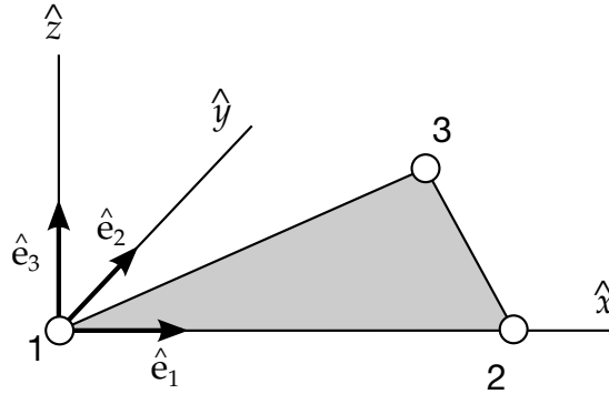
Figure 10.1. Local element coordinate system for C0 shell element.
