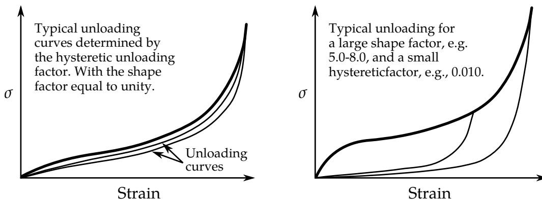
Figure 22.57.1. Behavior of the low-density urethane foam model.
