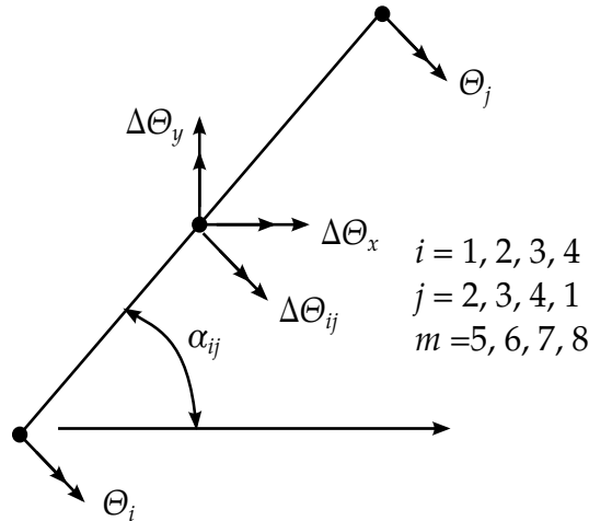
Figure 44.2. Element edge [Wilson, 2000]
