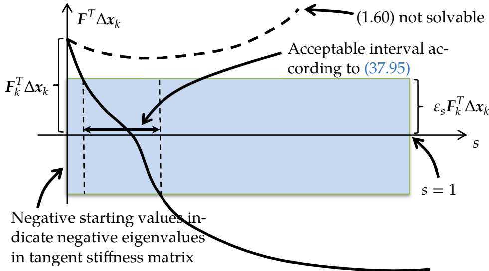
Figure 3737-4 Illustration of line search based on energy, may be complemented with norm of F . Dashed line indicates a line search that requires
