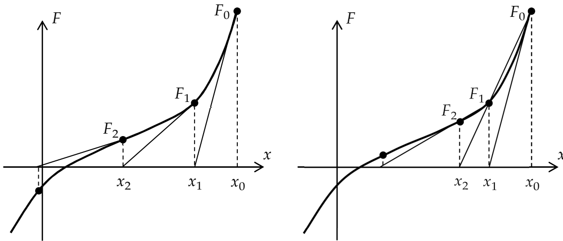
Figure 3737-2 Full Newton (left) compared to quasi-Newton secant updates (right), the linear approximation to obtain x_2 is for full Newton the exact tangent in (x_1, F_1) while it is the linear extension between the points (x_0, F_0) and (x_1, F_1)
