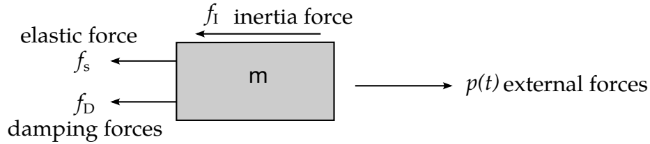
Figure 27.2. Forces acting on mass, m
