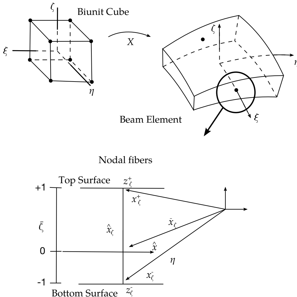
Figure 7.1. Hughes-Liu beam element.
