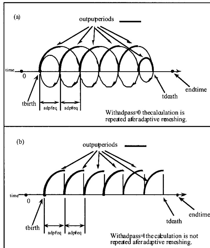
Figure 36.11. The input parameter, ADPASS, controls whether LS-DYNA backs up and repeats the calculation after adaptive refinement.
