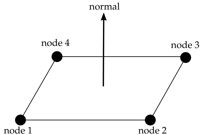
Figure 41.1. Counter-clockwise ordering of nodes when viewed from fluid looking towards solid provides unit normal vector pointing into the fluid.
