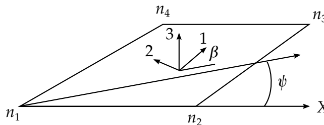
Figure 21.6. Orientation of material directions relative to the 1-2 side.
