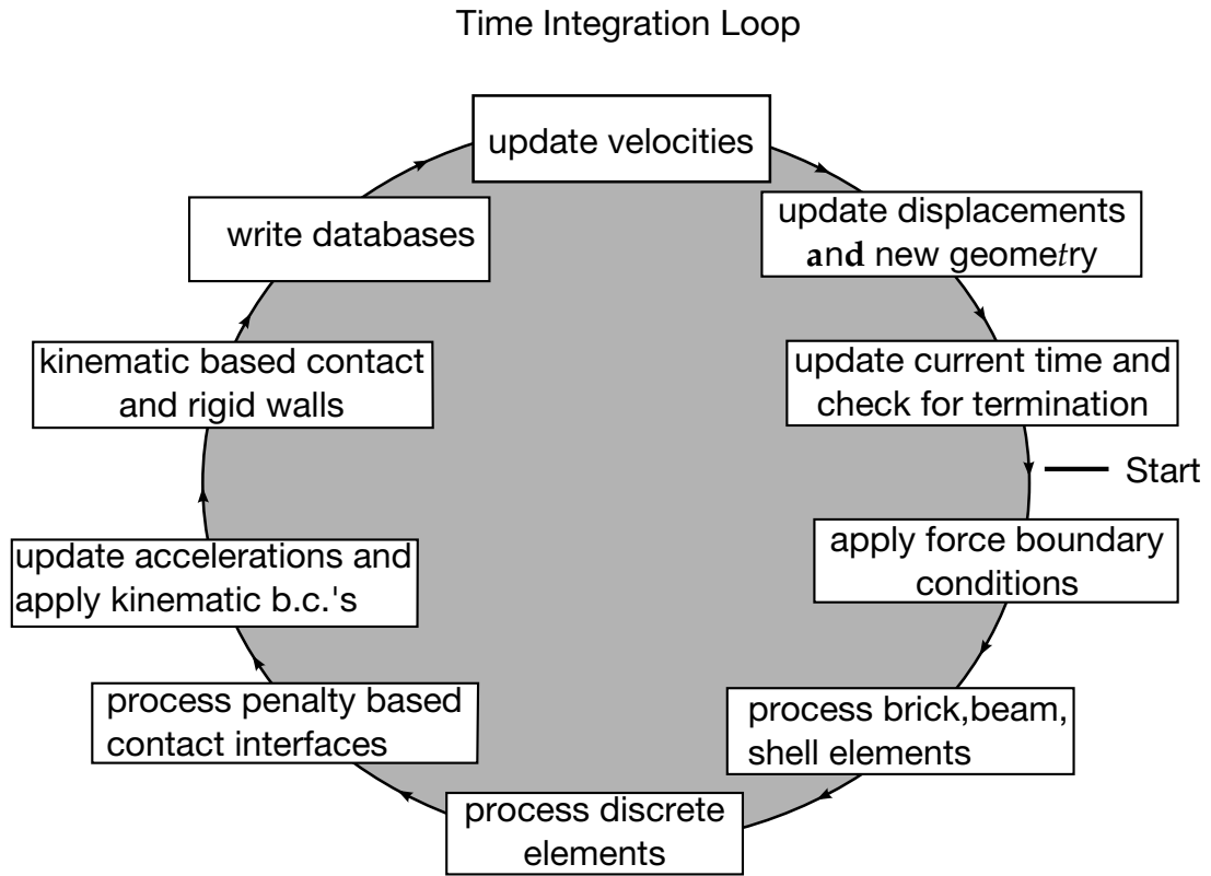
Figure 27.7. The time integration loop in LS-DYNA.
