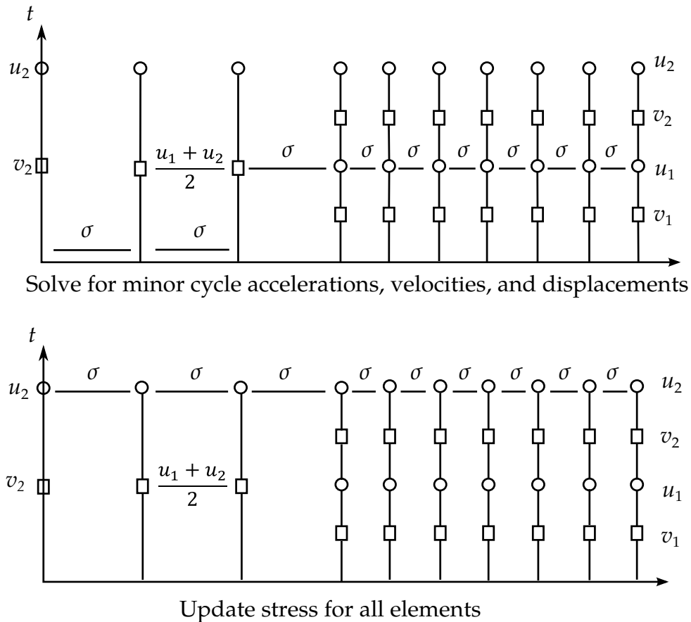
Figure 27.6. Timing diagram for subcycling algorithm based on linear nodal interpolations.
