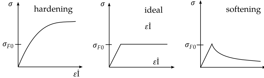
Figure 21.4. Hardening, ideal, and softening plasticity models.
