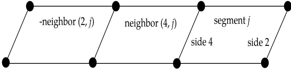
Figure 41.4. If neighbor (2, j) is a negative number it is assumed to lie on the opposite side of neighbor (4, j) as segment j .
