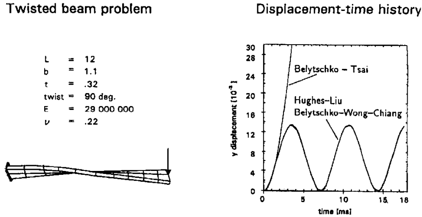
Figure 9.2. The twisted beam problem fails with the Belytschko-Tsay shell element.
