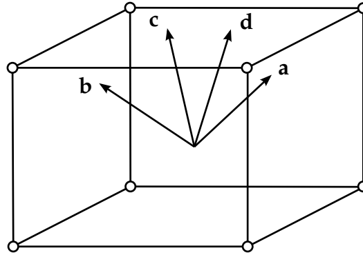
Figure 21.8. Local material directions are defined by a triad which can be input for each solid element.
