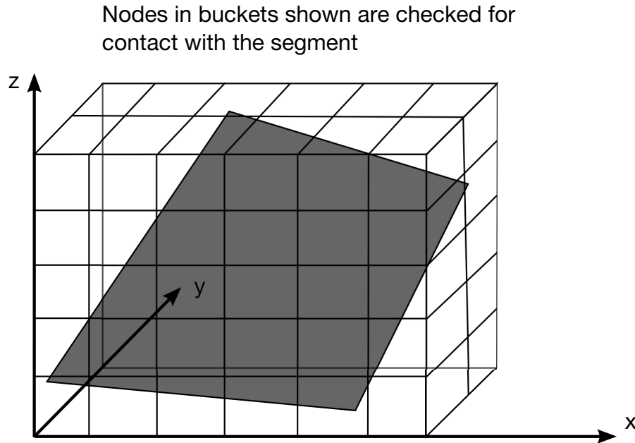
Figure 29.26. The orthogonal distance of each slave node contained in the box from the segment is determined. The box is subdivided into sixty buckets.
