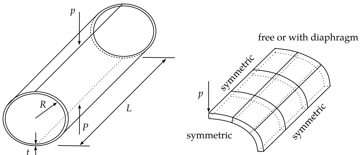
Figure 16.6. Pinched cylinder and the element model
