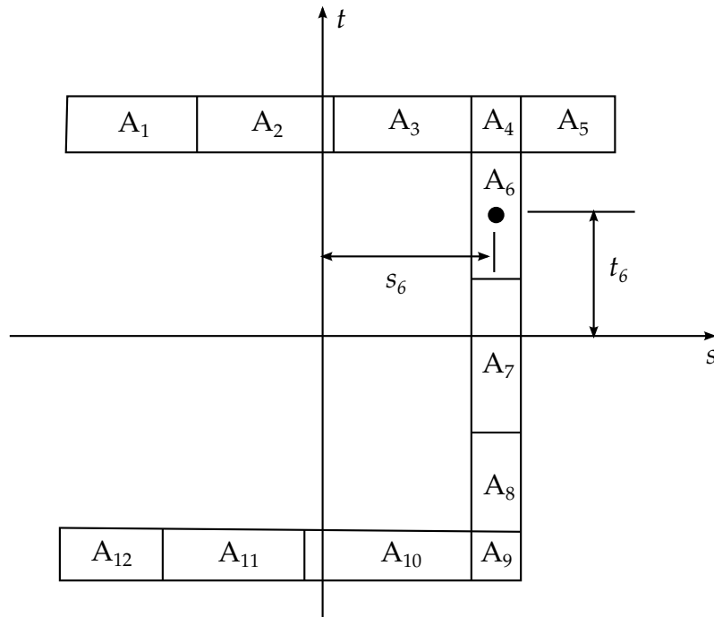
Figure 7.5. A breakdown of the cross section geometry in Figure 7.4 into twelve integration points.
