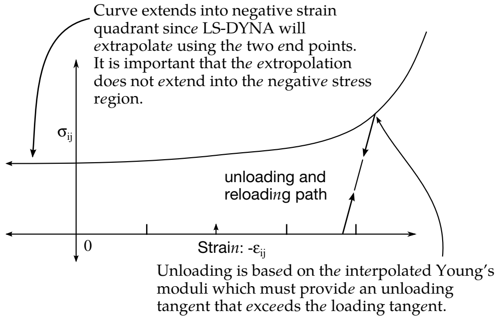
Figure 22.126.1. Stress quantity versus strain. Note that the “yield stress” at a strain of zero is nonzero. In the load curve definition the “time” value is the directional strain and the “function” value is the yield stress.
