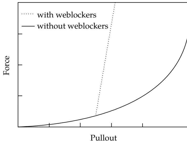
Figure 19.9. Retractor force pull characteristics.
