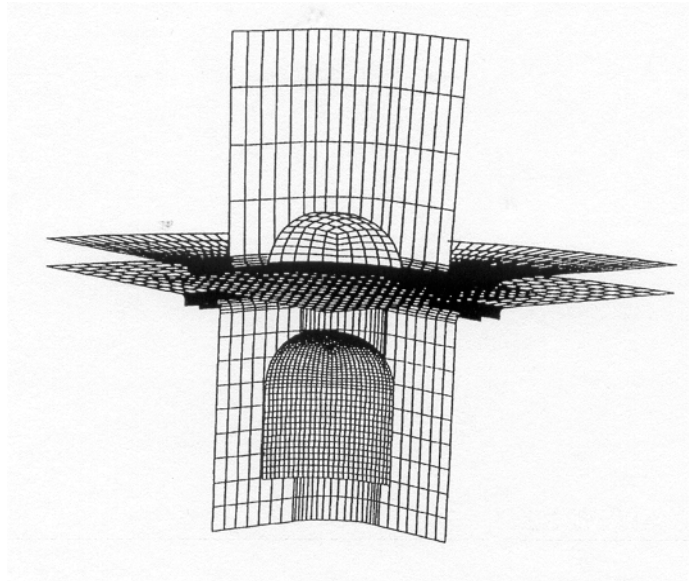
Figure 36.2. Aluminum blank with 400 shells in blank and four rigid tools.
