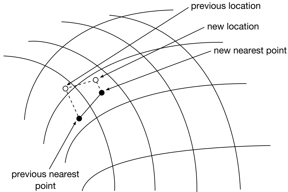
Figure 29.32. Newton iteration solves for the nearest point on the analytical surface.
