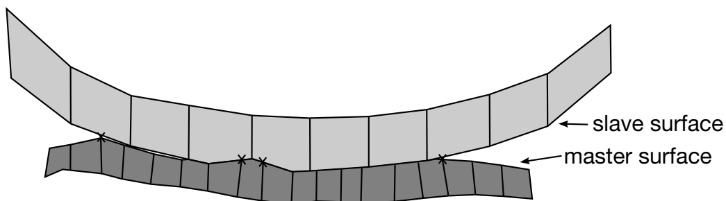
Figure 29.1. Nodes of the master slide surface designated with an “x” are treated as free surface nodes in the nodal constraint method.
