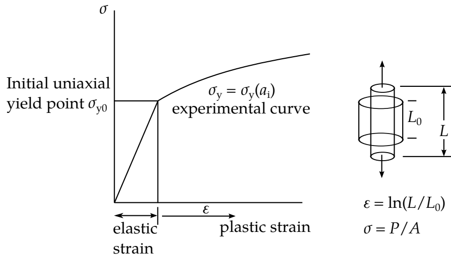
Figure 21.1. The uniaxial tension test demonstrates plastic behavior.
