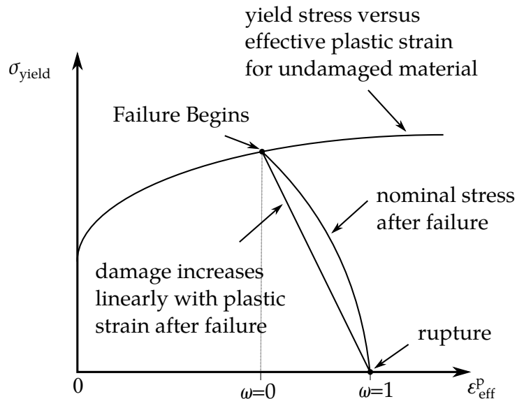
Figure .22.81.1. Stress strain behavior when damage is included.
