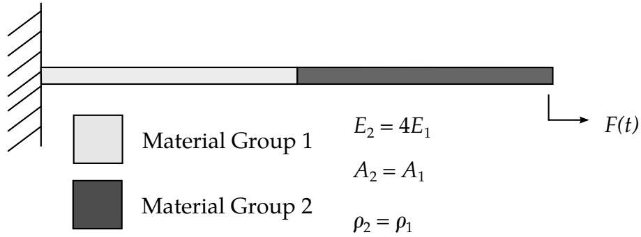
Figure 27.4. Subcycled beam problem from Hulbert and Hughes [1988].
