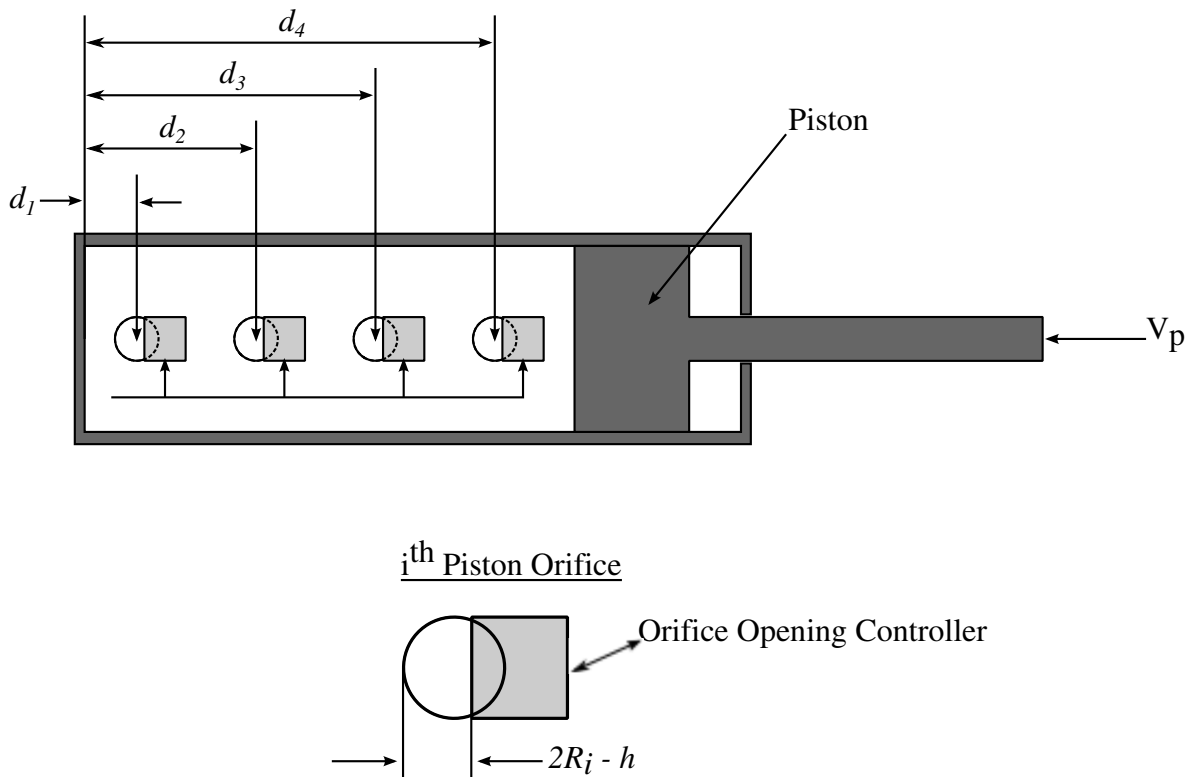
Figure 22.69.1. Mathematical model for the Side Impact Dummy damper.
