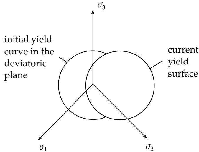
Figure 21.3. With kinematic hardening the yield surface may shift as a function of plastic strain.
