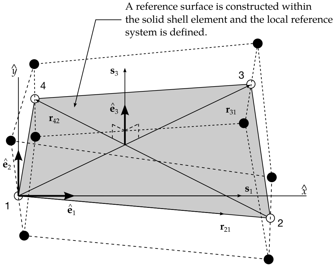
Figure 15.2. Construction of the reference surface in the solid shell element.
