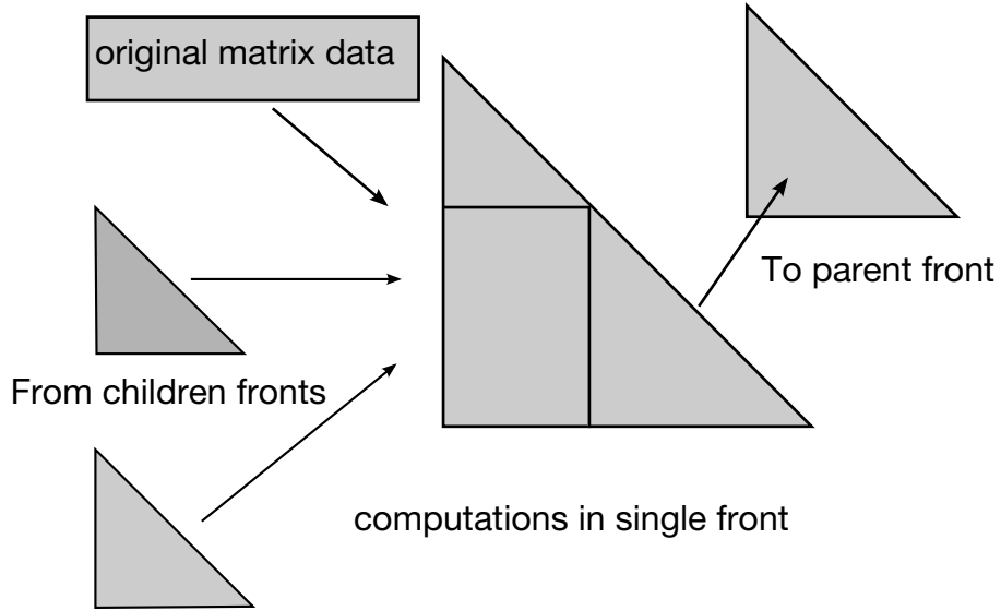
Figure 39.2. Single front algorithm.
