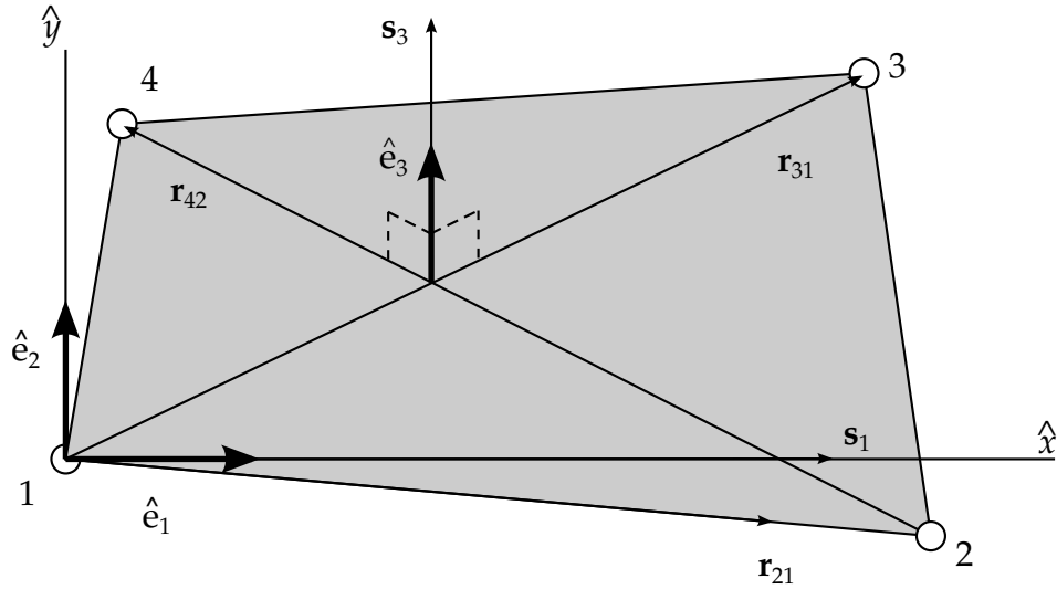
Figure 9.1. Construction of element coordinate system is shown.
