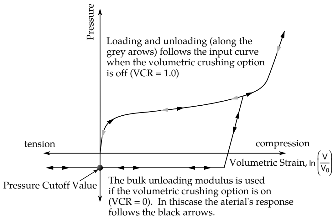
Figure 22.5.1. Volumetric strain versus pressure curve for soil and crushable foam model.
