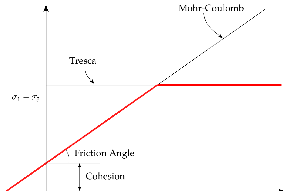
Figure 22.16.1. Mohr-Coulomb surface with a Tresca limit.
