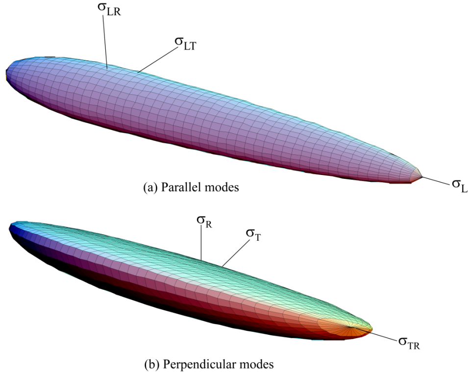
Figure 22.143.1. The yield criteria for wood produces smooth surfaces in stress space.
