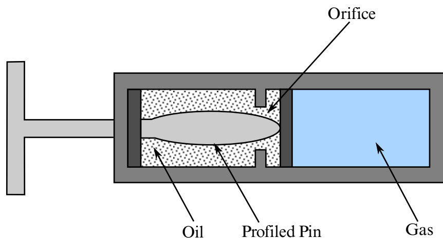
Figure 22.70.1. Schematic of Hydraulic/Gas damper.
