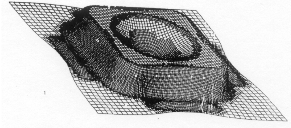
Figure 36.4. Final shape of formed part with 4315 shell elements per quarter.
