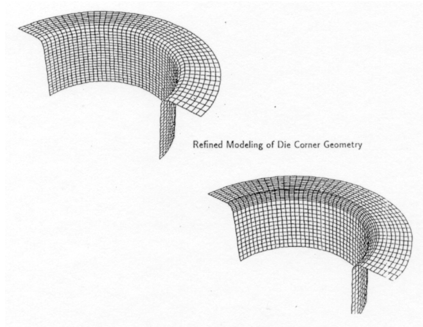
Figure 29.18. Refinement of die radius.
