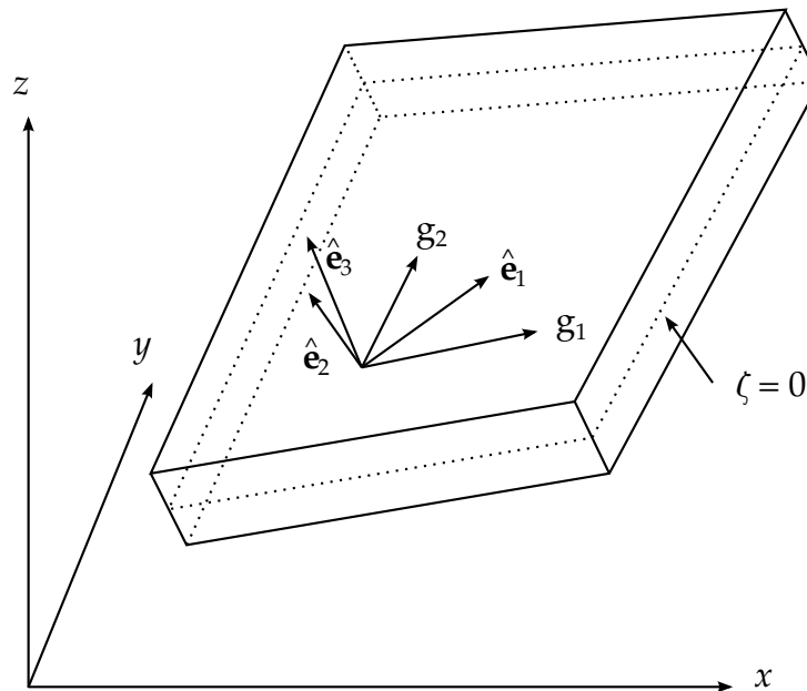
Figure 16.1. Definition of co-rotational coordinate system
