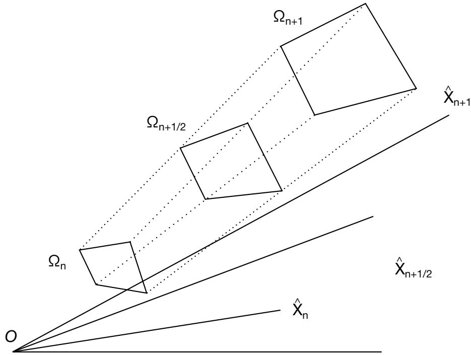
Figure 16.2. Configurations at times t_n , t_{n+\frac{1}{2}} and t_{n+1} ,
