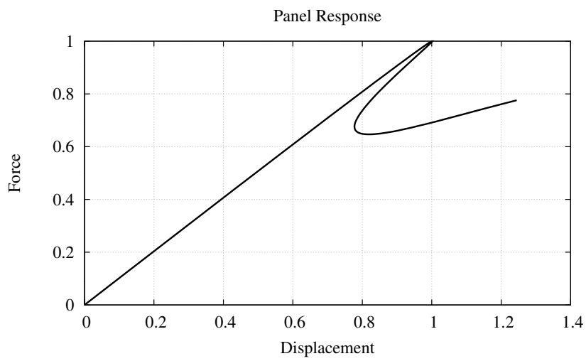
Figure 38-3 Snap-back buckling of panel, normalized force displacement curve shown
