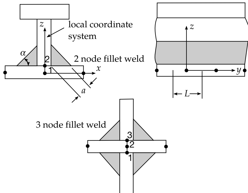
Figure 28.3. Nodal ordering and orientation of the local coordinate system is shown for fillet weld failure.
