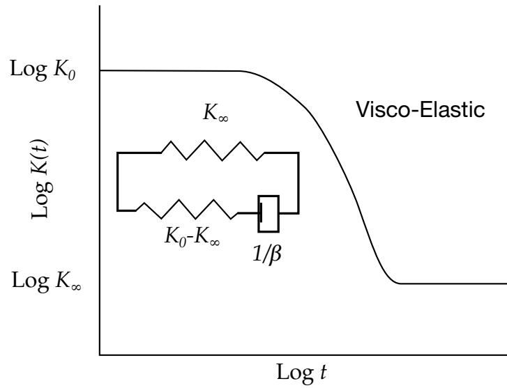
Figure 19.4. Typical stiffness relaxation curve used for the viscoelastic discrete element.
