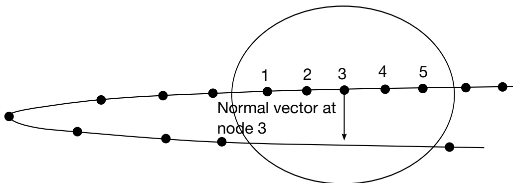
Figure 29.25. Nodes 2 and 4 share segments with node 3 and therefore the two nearest nodes are 1 and 5. The nearest contact segment is not considered since its nodes are not members of the nearest node set.
