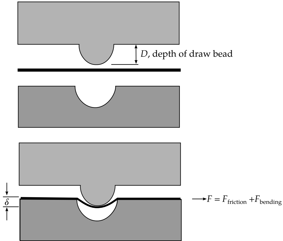
Figure 29.36. Draw bead contact model defines a resisting force as a function of draw bead displacement.
