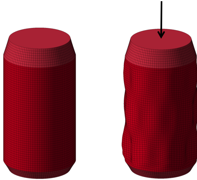
Figure 3737-1 Linear axial buckling of an aluminium beverage can.
