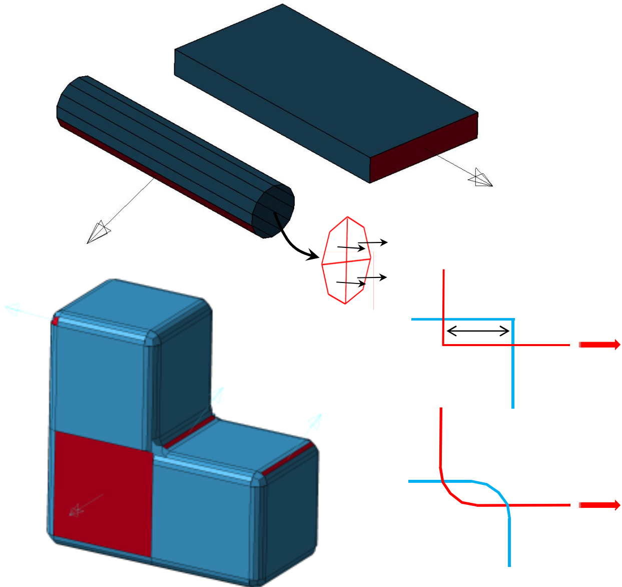
Figure 29-42 29 Faceted representation of beams (including 4 quads representing a tip end), shell and sharp solid edges, respectively, the segment geometry indicated by red. The contact surface representation of three cubic solid elements is illustrated, with a somewhat exaggerated smoothing for illustration purposes. The effect of edge smoothing in contact is illustrated in a section cut bottom right, if the red objects slides to the right and the blue objects are fixed, the sudden detection of a parasitic contact indicated by the double arrow results in a jump in the contact force, this is alleviated by smoothing of the edges below.
