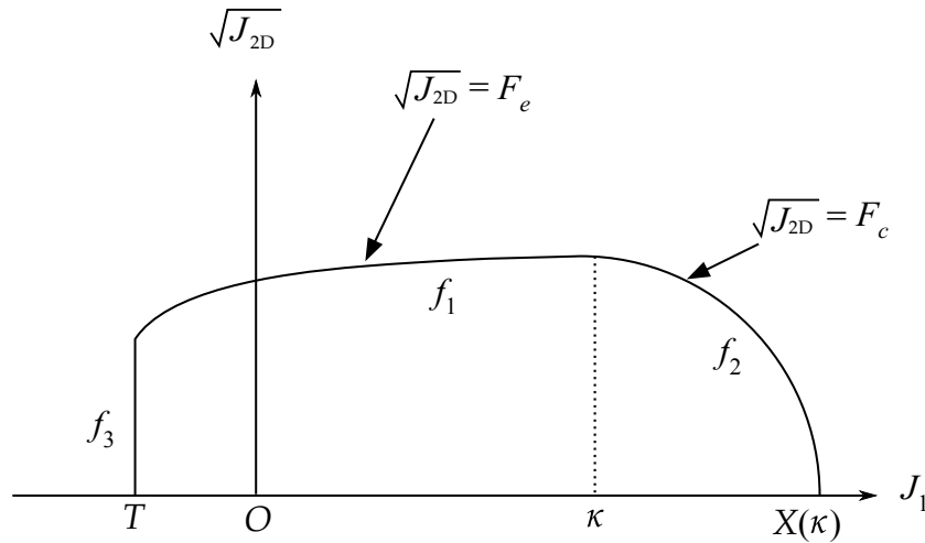
Figure 22.25.2. The yield surface of the two-invariant cap model in pressure \sqrt{J_{2D}} - J_1 space. Surface f_1 is the failure envelope, f_2 is the cap surface, and f_3 is the tension cutoff.
