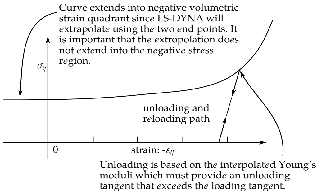
Figure 22.26.1. Stress quantity versus volumetric strain. Note that the “yield stress” at a volumetric strain of zero is nonzero. In the load curve definition, the “time” value is the volumetric strain and the “function” value is the yield stress.
