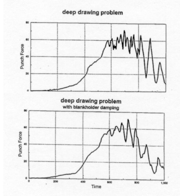
Figure 29.17. Reaction forces with and without contact damping.
