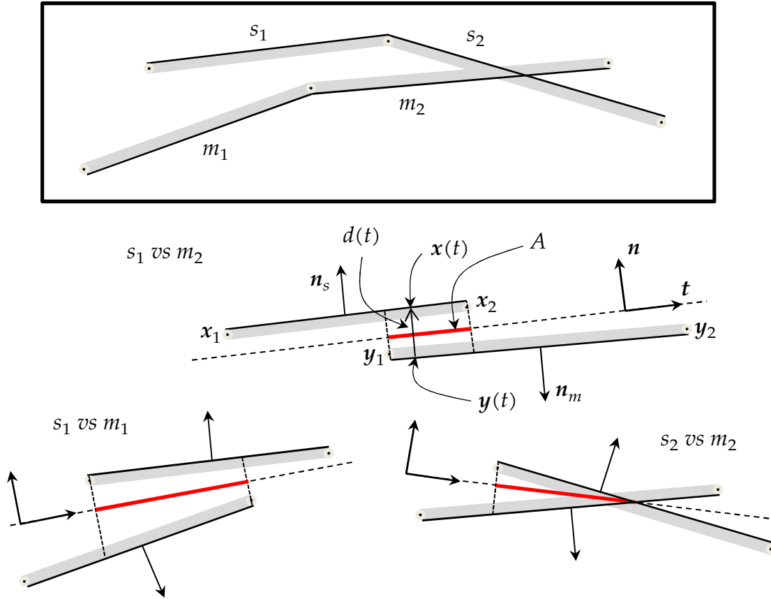
29-4629 2D mortar contact, 2 slave segments in contact with 2 master segments results in three separate treatments.
