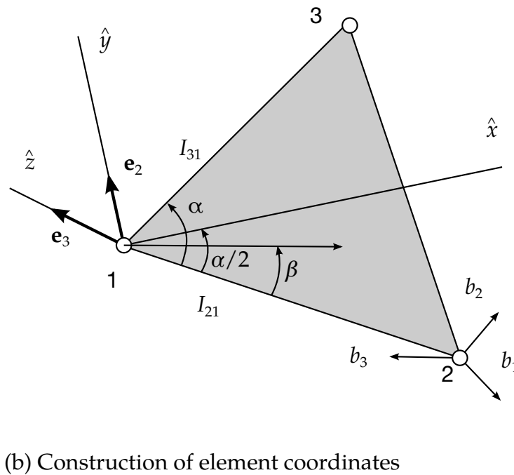
Figure 10.3. Construction of local element coordinate system.
