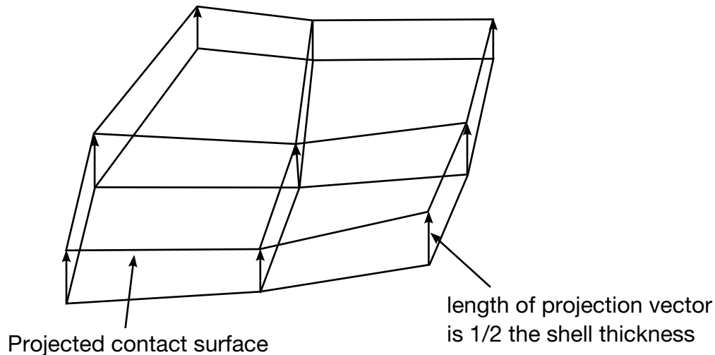
Figure 29.11. Contact surface is based on mid-surface normal projection vectors.
