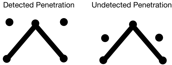
Figure 29.14. Undetected interpenetration. Such interpenetrations are frequently due to the use of coarse meshes.
