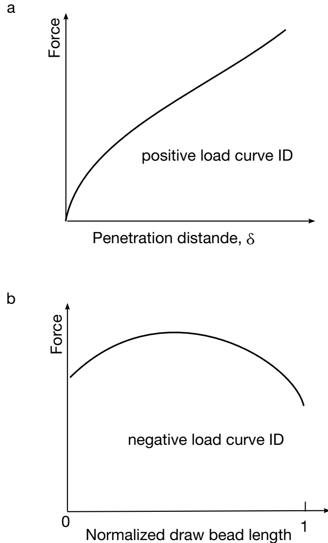
Figure 29.35. Draw bead contact model defines a resisting force as a function of draw bead displacement.
