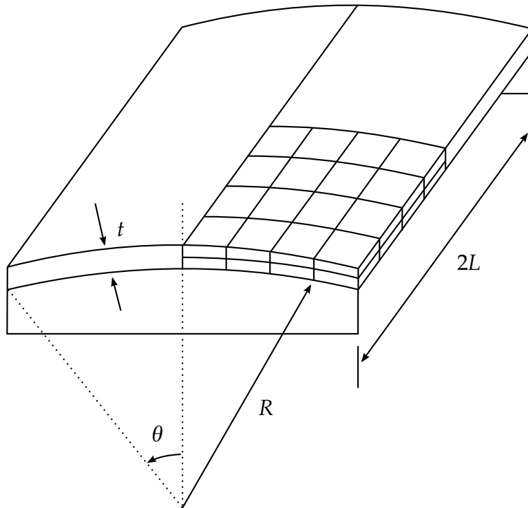
Figure 16.7. Scordelis-Lo roof under self-weight
