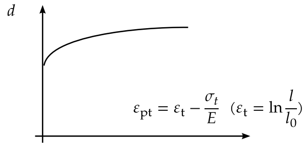
Figure 22.4. Damage parameter from uniaxial tensile test
