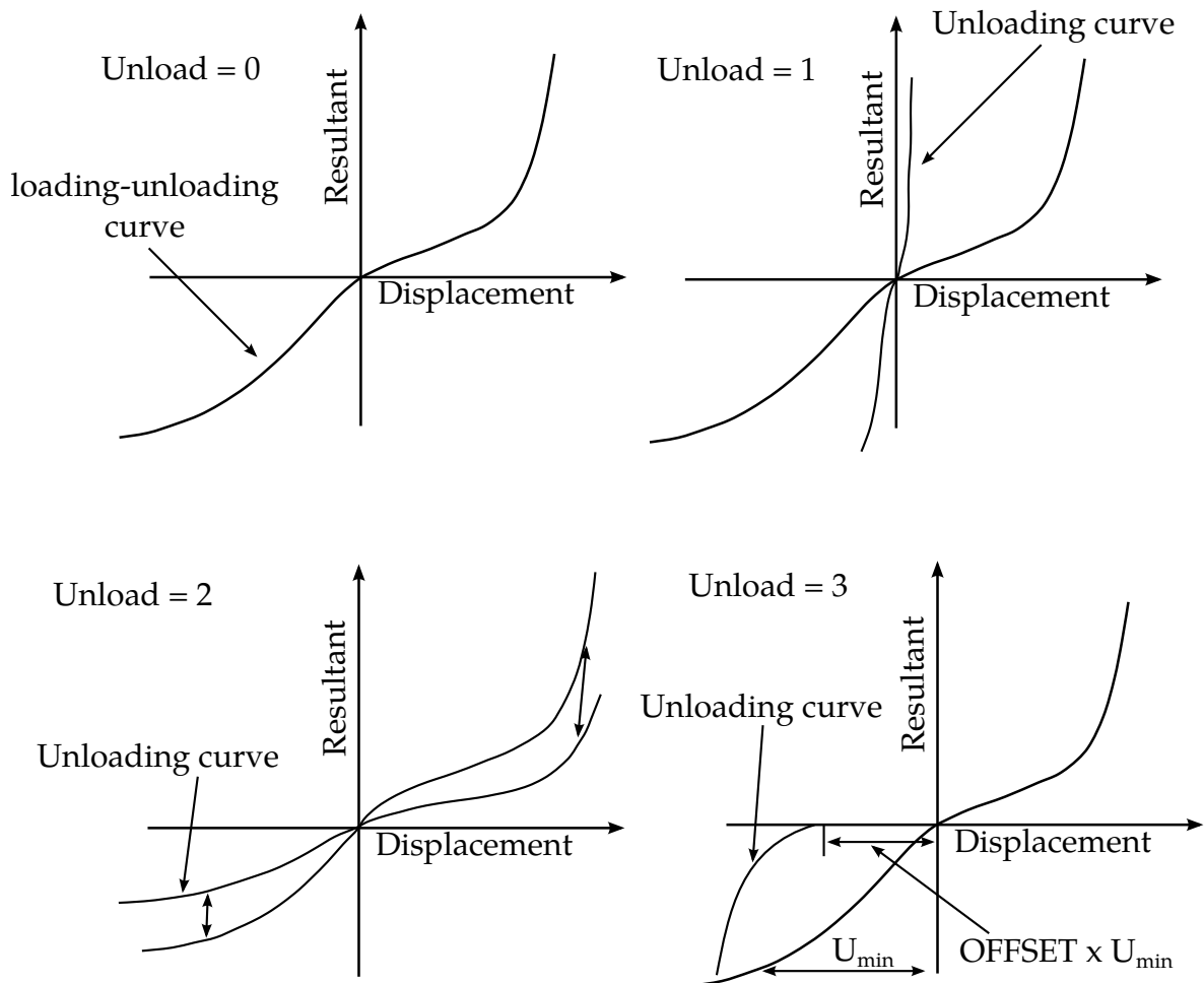
Figure 22.119.1. Load and unloading behavior.
