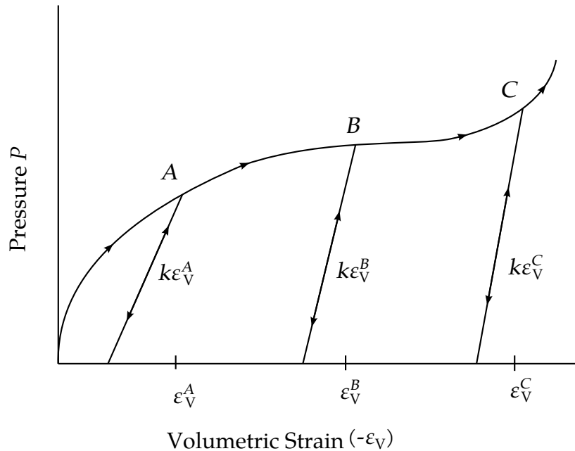
Figure 23.1. Pressure versus volumetric strain curve for equation of state form 8 with compaction. In the compacted states, the bulk unloading modulus depends on the peak volumetric strain.
