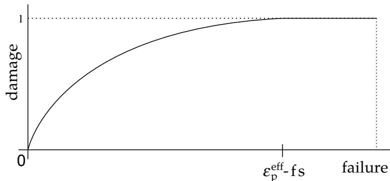
Figure 22.81.2. A nonlinear damage curve is optional. Note that the origin of the curve is at (0,0). It is permissible to input the failure strain, fs , as zero for this option. The nonlinear damage curve is useful for controlling the softening behavior after the failure strain is reached.
