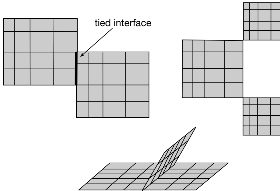
Figure 29.23. Incremental searching may fail on surfaces that are not simply connected. The new contact algorithm in LS-DYNA avoids incremental searching for nodal points that are not in contact and all these cases are considered.
