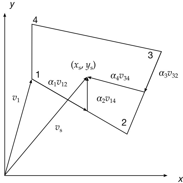
Figure 20.2. Skew Coordinate System
