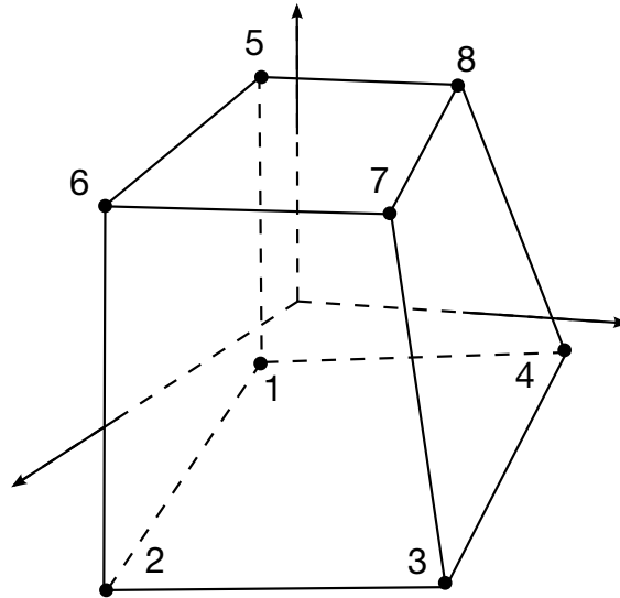
Figure 21.9. The orientation of the triad for the local material directions is stored relative to the base of the solid element. The base is defined by nodes 1-4 of the element connectivity.
