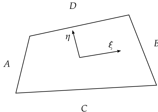
Figure 11.1. Midside locations of isoparametric strain rates
