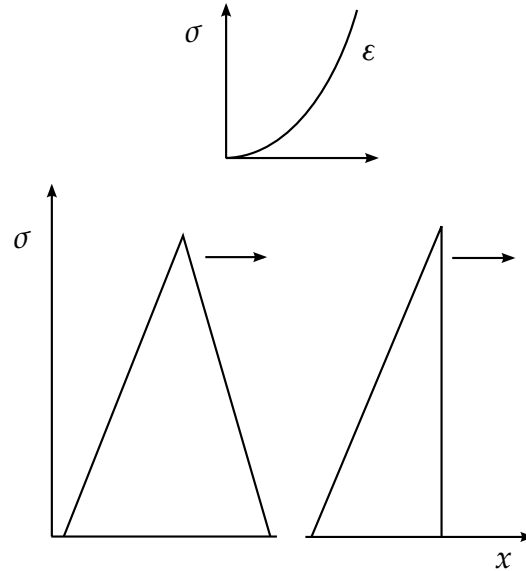
Figure 24.1. If the sound speed increases as the stress increases the traveling wave above will gradually steepen as it moves along the x -coordinate to form a shock wave.
