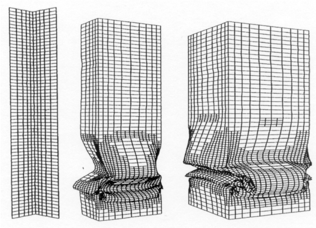
Figure 36.1. One level adaptive calculation on a square cross section beam.
