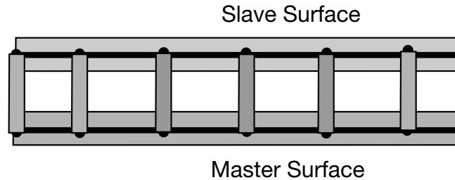
Figure 29.21. Offset tied interface.
