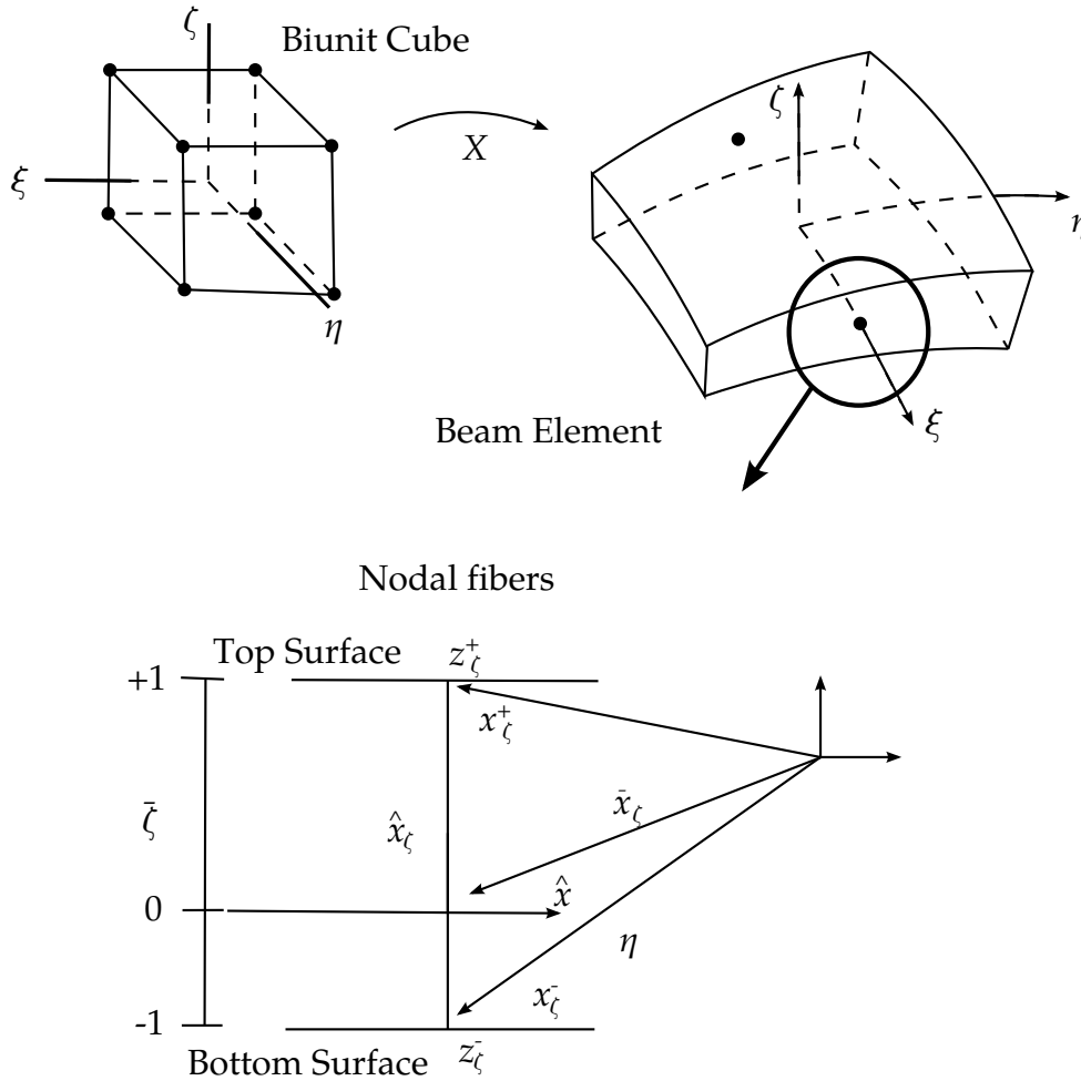
Figure 13.1. Mapping of the biunit cube into the Hughes-Liu shell element and nodal fiber nomenclature.
