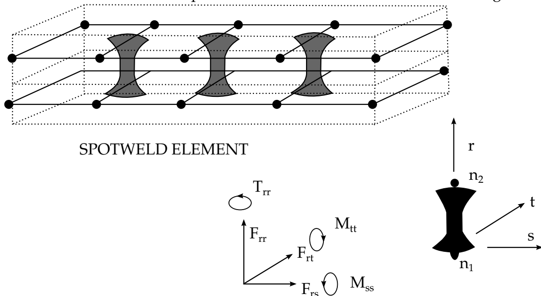
Figure 22.100.1. Deformable spotwelds can be arbitrarily placed within the structure.
