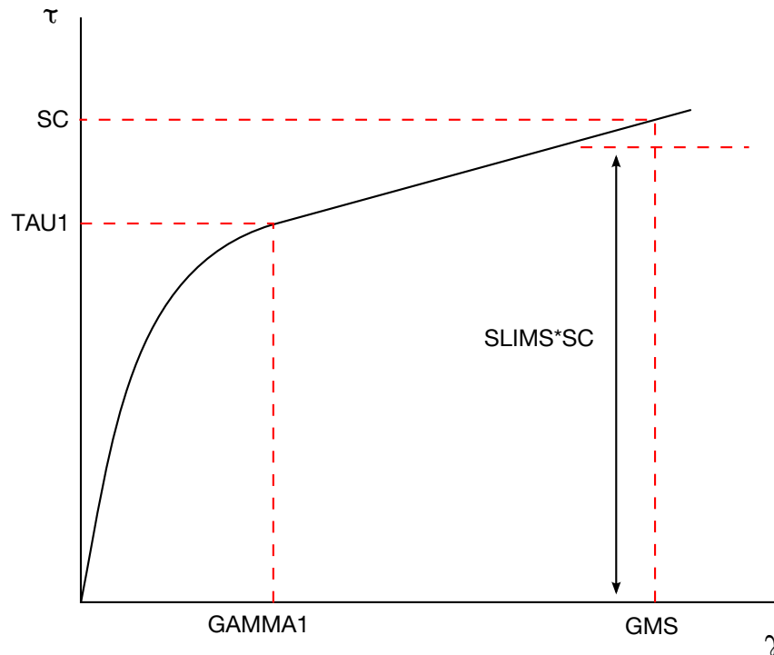
Figure 22.58.1. Stress-strain diagram for shear.
