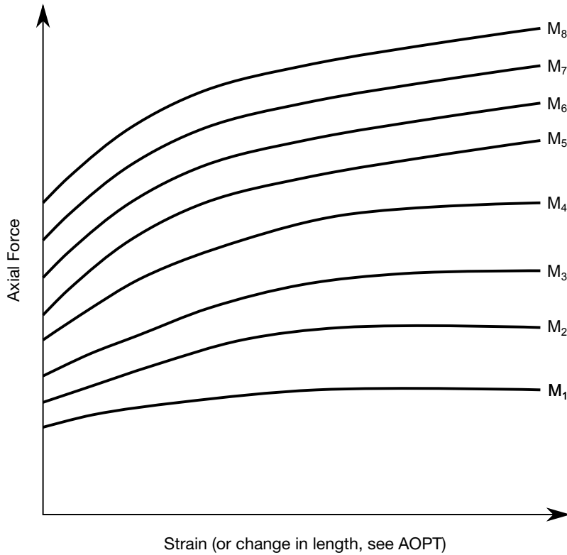
Figure 22.29.1. The force magnitude is limited by the applied end moment. For an intermediate value of the end moment, LS-DYNA interpolates between the curves to determine the allowable force.
