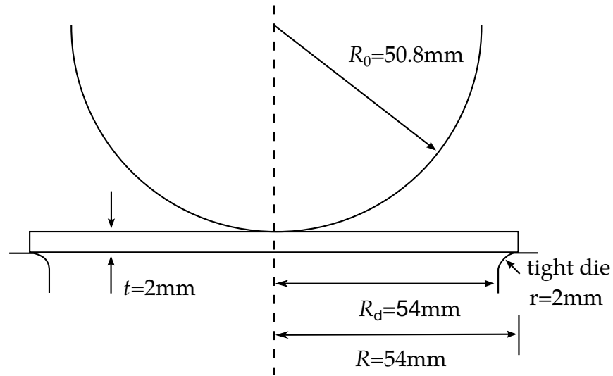
Figure 16.8. Circular sheet stretched with a tight die
