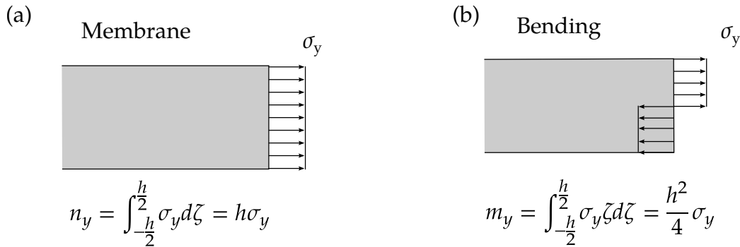
Figure 22.28.1. Full section yield using resultant plasticity.
