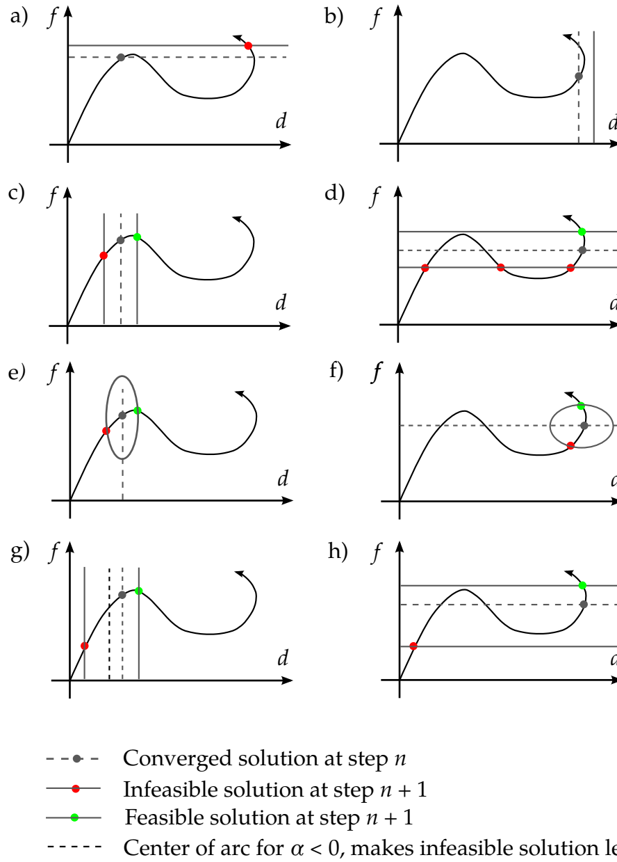
Figure 38.1. Representative force-displacement curves for illustrating arc-length and accompanying parameters
