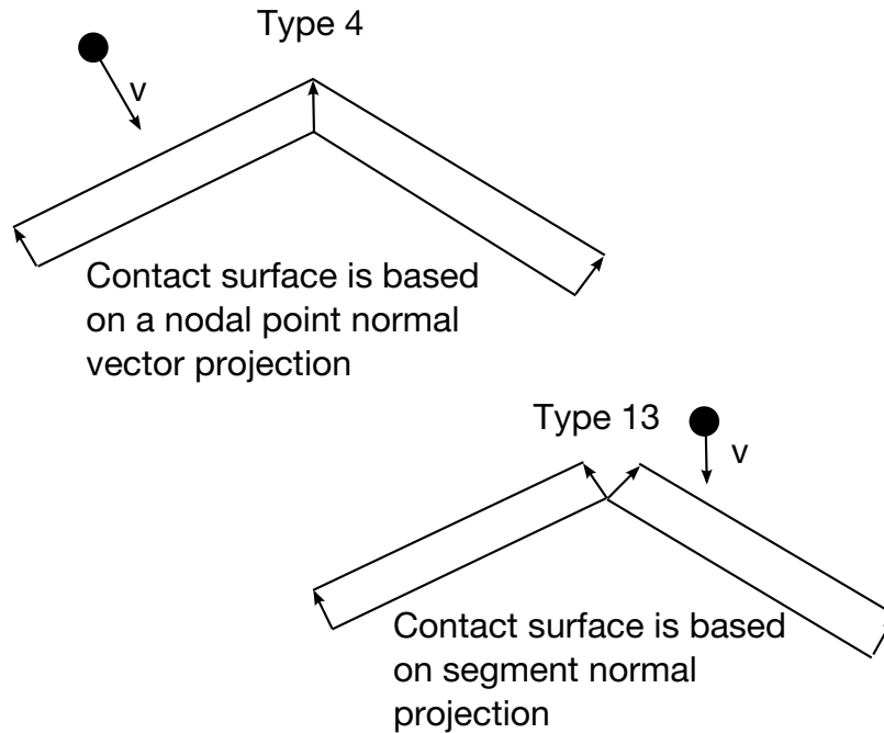
Figure 29.27. Projection of the contact surface for a node approaching from above is shown for types 4 and 13 contact.
