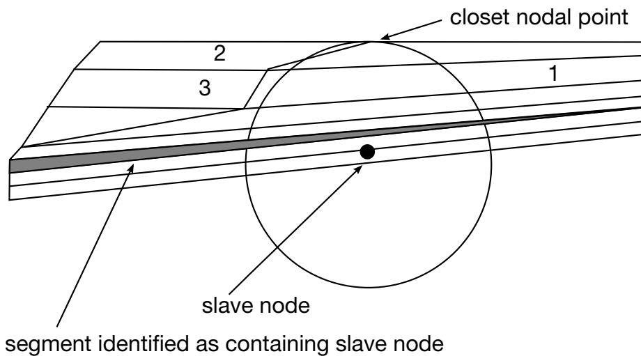
Figure 29.10. In case the stored segment fails to contain the node, the adjacent segments are checked.
