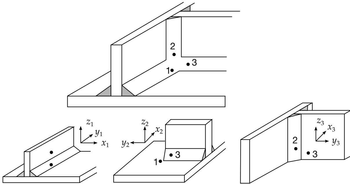
Figure 28.5. A simple cross fillet weld illustrates the required input. Here NFW = 3 with nodal pairs (A = 2, B = 1) , (A = 3, B = 1) , and (A = 3, B = 2) . The local coordinate axes are shown. These axes are fixed in the rigid body and are referenced to the local rigid body coordinate system which tracks the rigid body rotation.
