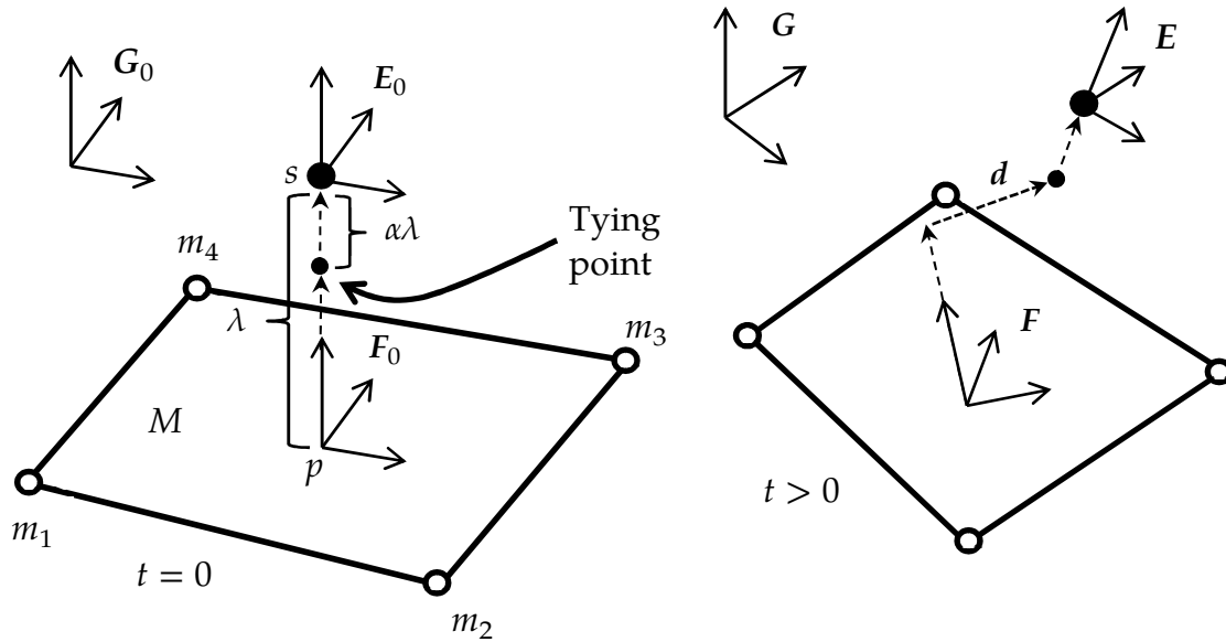
Figure 2929-22 Kinematics of the implicit strong objective tied contact formulation
