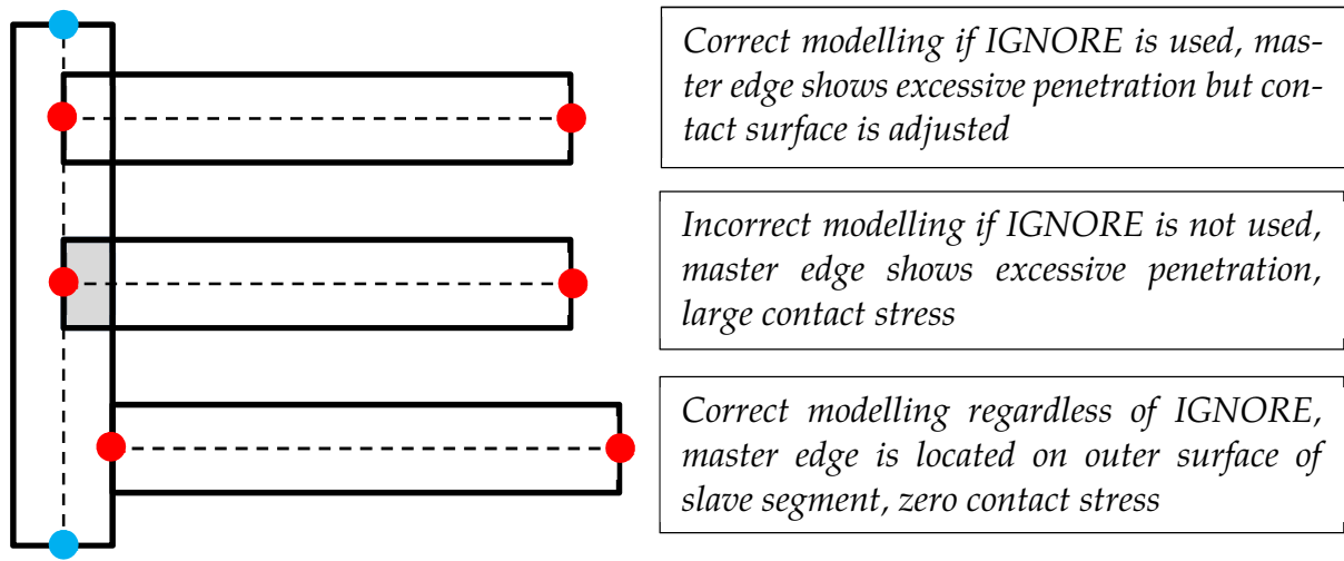
Figure 29-43 Intersected view of shells in edge-to-surface contact. Shell mid-surfaces indicated by dashed lines, outer surfaces by solid lines. Slave shell nodes are blue, master shell nodes are red and initial volume of penetration is shaded.
