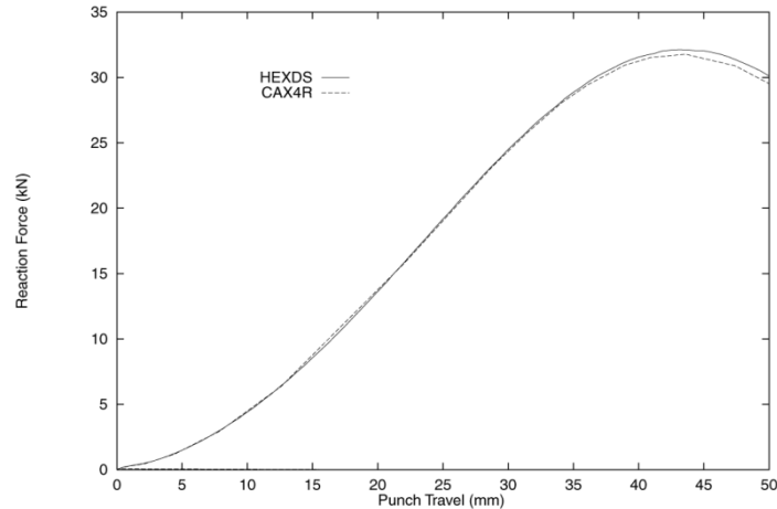
Figure 16.11. Reaction force vs. punch travel for the circular sheet
