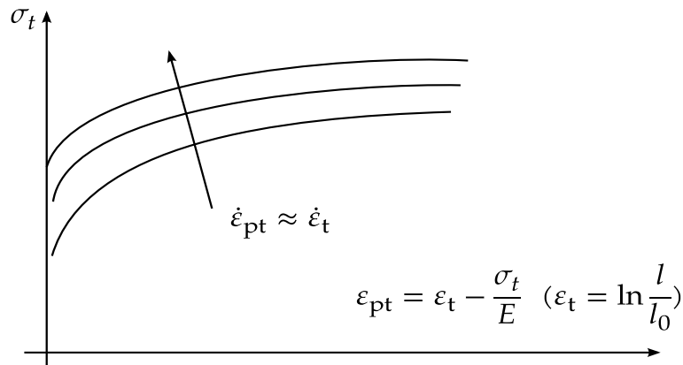
Figure 22.3. Tensile hardening curve from dynamic tensile tests
