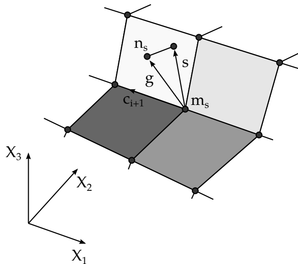
Figure 29.4. Projection of \mathbf{g} onto master segment s_1
