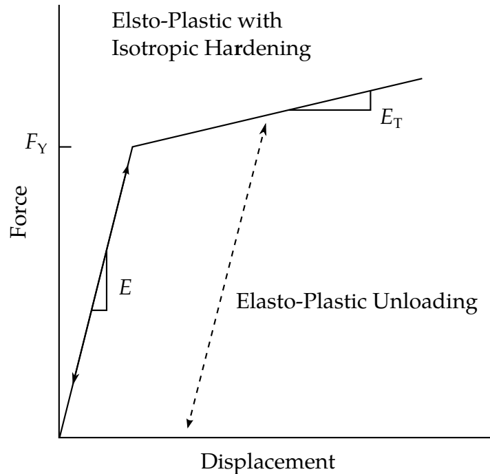
Figure 19.2. Loading and unloading force-displacement curves for elasto-plastic discrete element.
