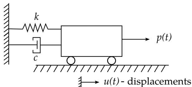
Figure 27.1. Single degree of freedom damped system.
