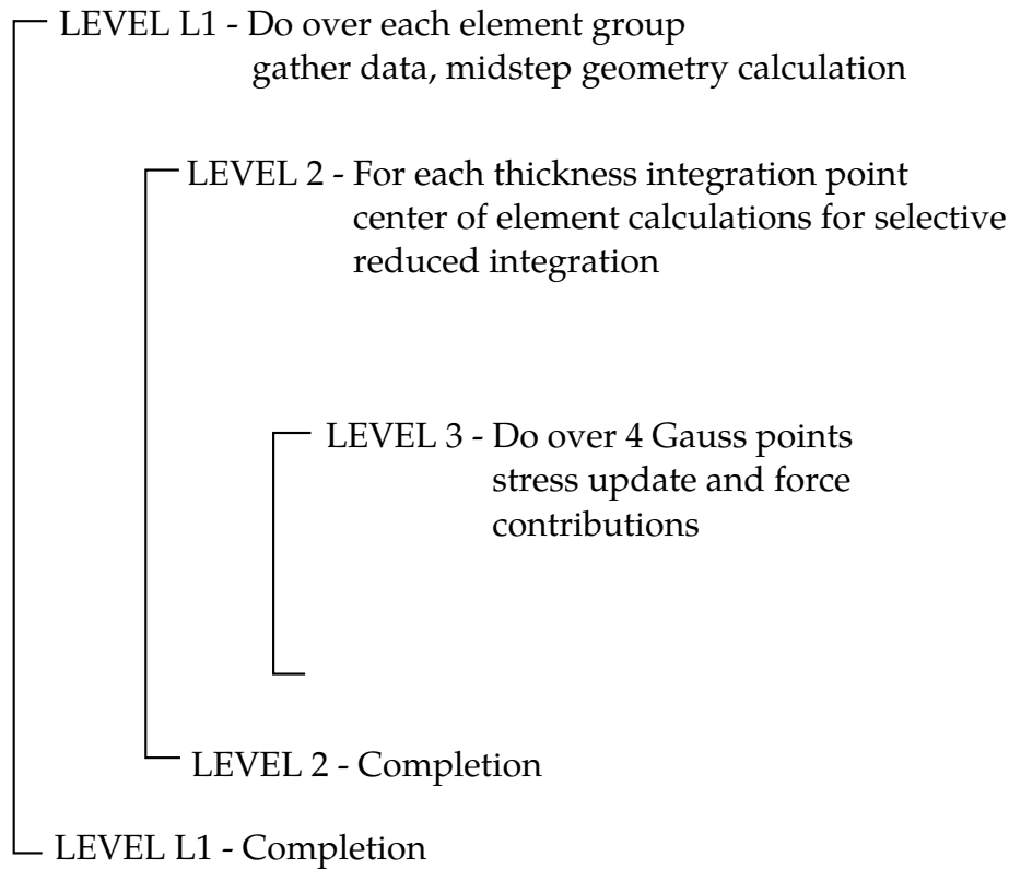
Figure 13.6. An inner loop, LEVEL 3, is added for the Hughes-Liu shell with selectively reduced integration.
