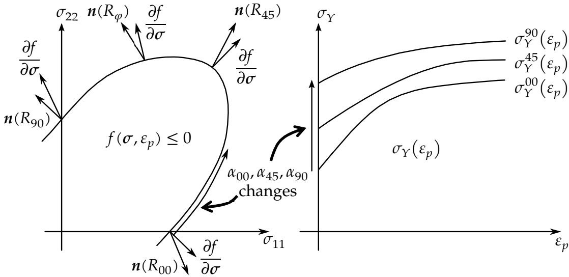
22-1 Plastic flow direction (left) and hardening (right) illustrated for variable R-values and hardening. Changes in \alpha_{00}, \alpha_{45} and \alpha_{90} come from changes
