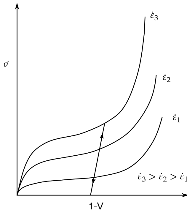
Figure 22.163.1. Rate effects are defined by a family of curves giving yield stress versus volumetric strain.
