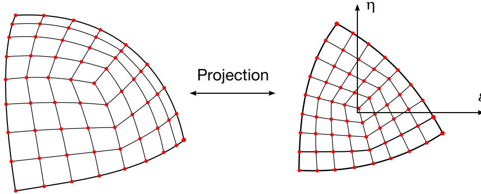
Figure 43.2. Mesh-free shell global approach
