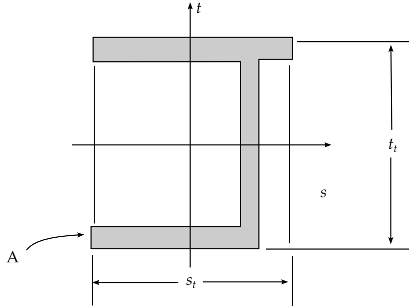
Figure 7.4. Specification of the nodal thickness, s_t and t_t , for a beam with an arbitrary cross-section.
