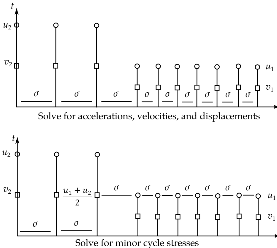
Figure 27.5. Timing diagram for subcycling algorithm based on linear nodal interpolations.
