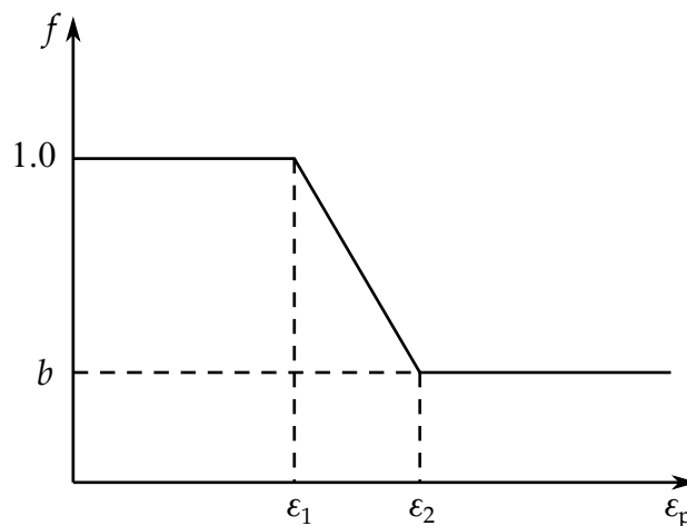
Figure 22.78.1. Strength reduction factor.
