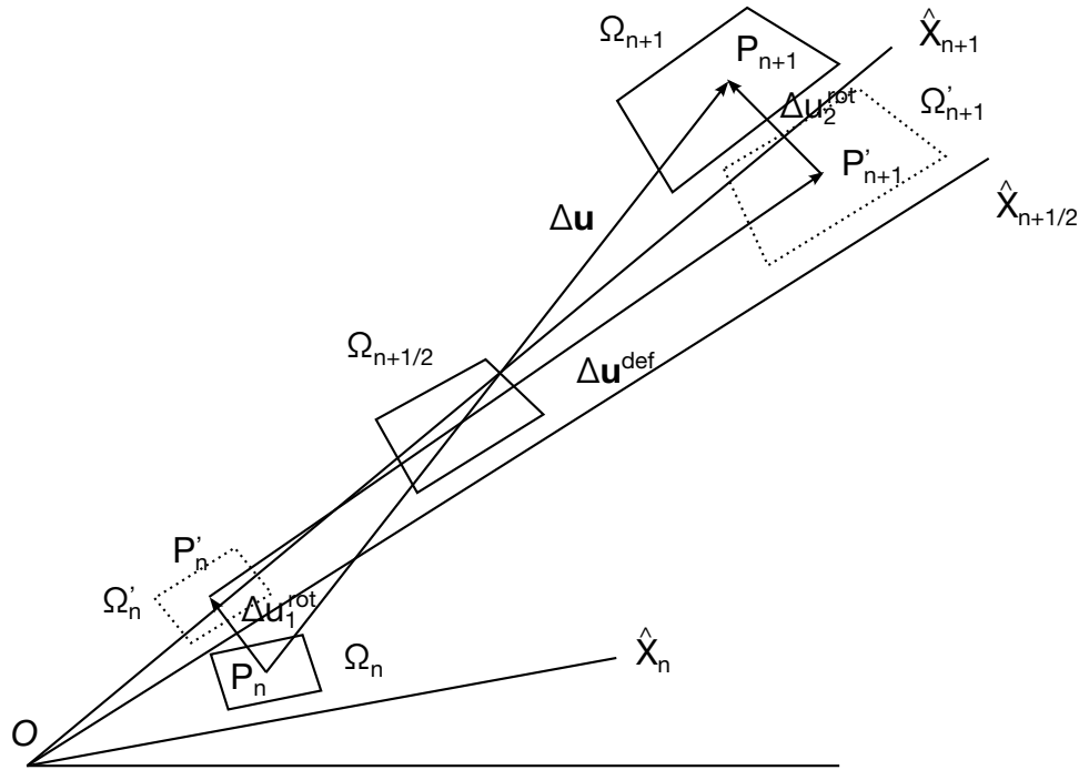
Figure 16.3. Separation of the displacement increment
