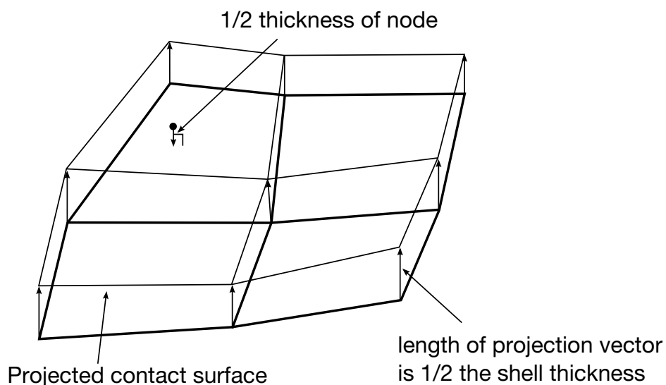
Figure 29.13. In a type 5 contact, thickness can also be taken into account.
