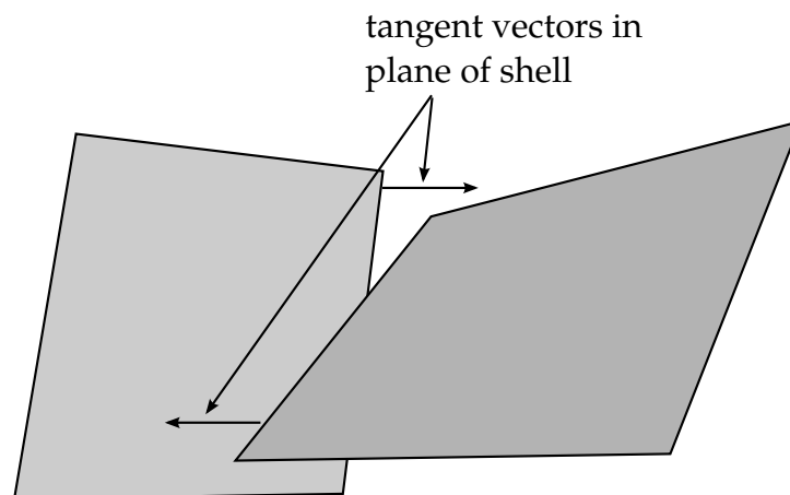
Figure 29.38. Single edge contact considers contact between two edges whose normals point towards each other.
