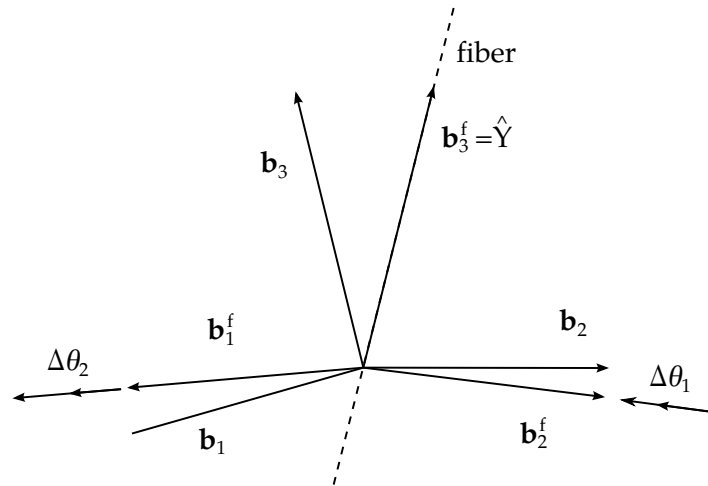
Figure 13.3. Incremental update of fiber vectors using Hughes-Liu incremental rotations.
