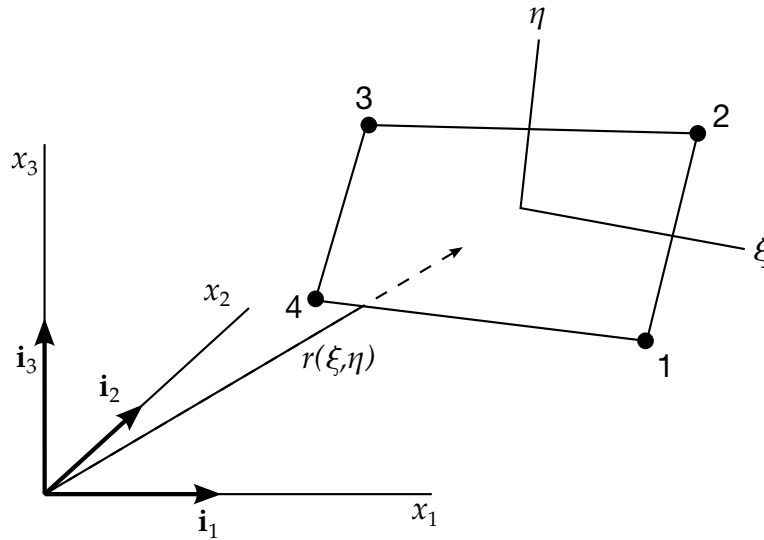
Figure 26.1. Parametric representation of a surface segment.
