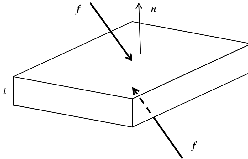
Figure 1212-2 Contact influence on thickness stretch shells.
