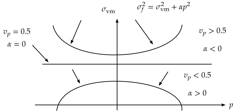
Figure 22.2. Influence of the flow rule on the plastic Poisson ratio
