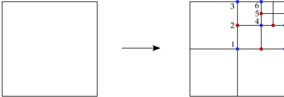
Figure 36.9. Illustration of which nodes are constrained after adaptive steps. The red nodes are dependent while the blue nodes constrain the dependent node that shares the edge.
