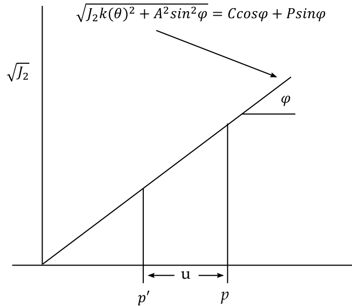
Figure 22.147.2. The effect on pressure due to pore water pressure.
