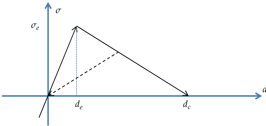
Figure 5.2. Common stress versus separation for a cohesive interface
