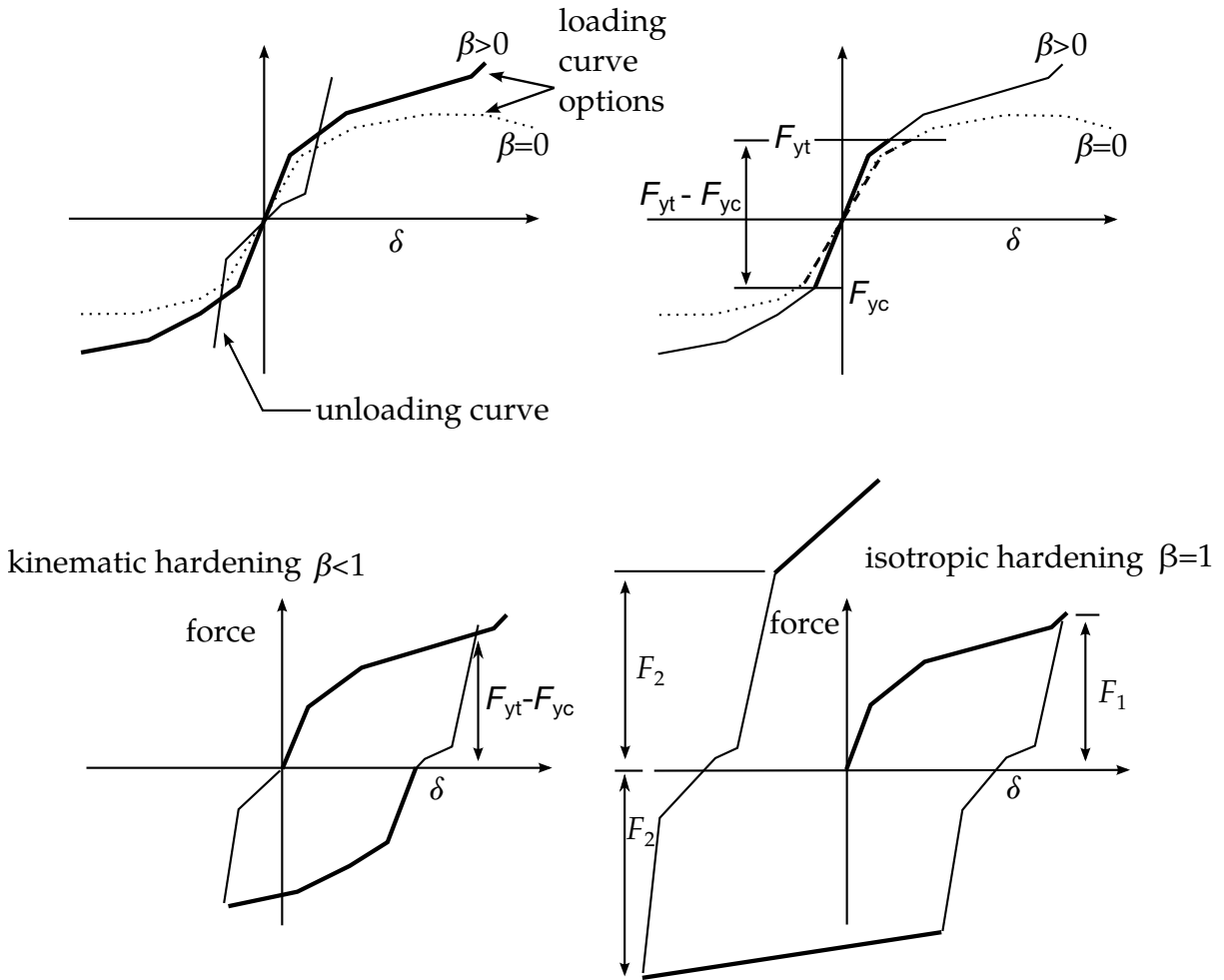
Figure 19.3. Loading and unloading force displacement curves for general non-linear discrete element.
