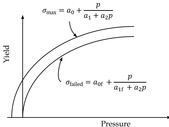
Figure 22.2. Two-curve concrete model with damage and failure.
