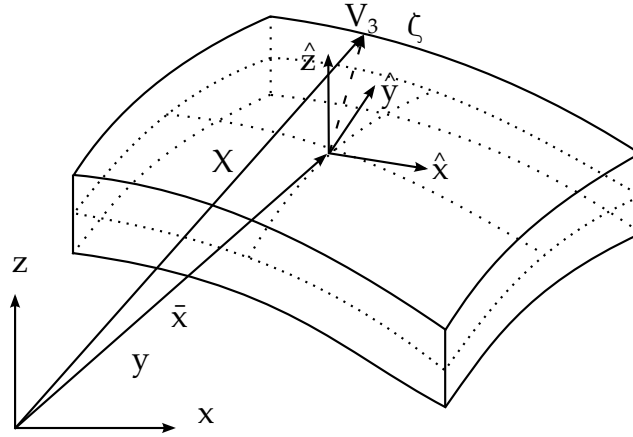
Figure 43.4. Geometry of a shell.
