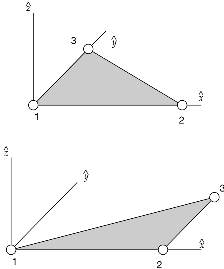
Figure 10.2. Element configurations with node 3 aligned with node 1 (left) and node 3 aligned with node 2 (right).
