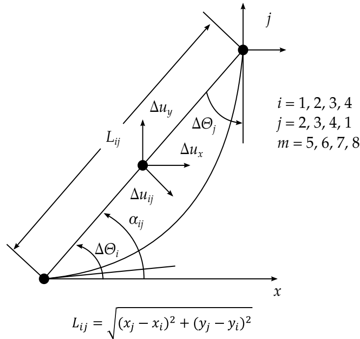
Figure 44.5. Corner node drilling rotations and mid side edge normal displacement [Wilson, 2000].
