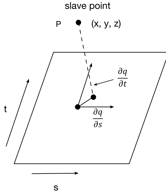
Figure 29.31. The geometry of the patch is a function of the parametric coordinates s and t .
