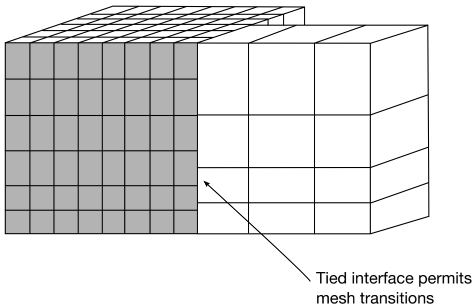
Figure 29.20. Tied interface used for a mesh transition.
